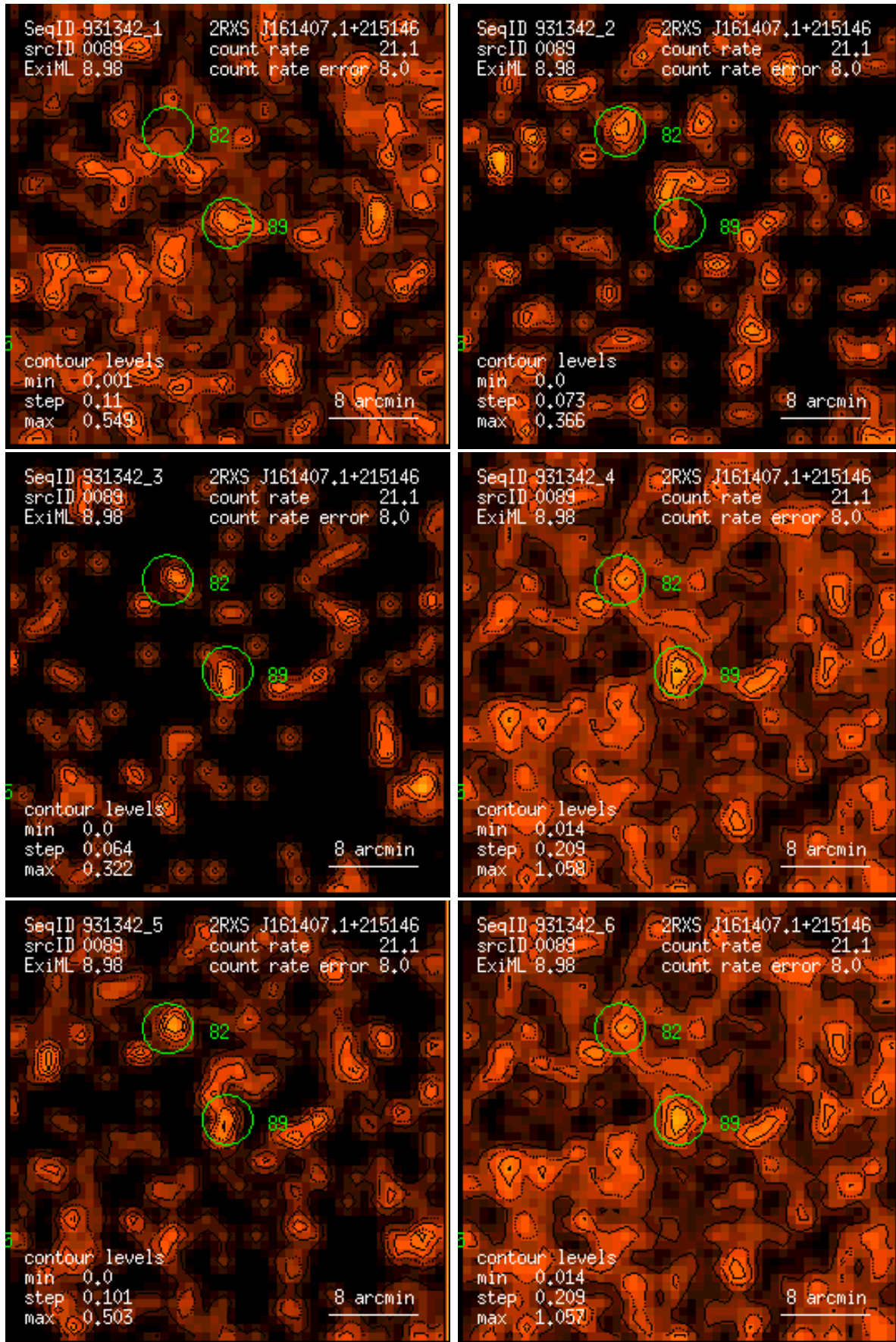
Figure 89: RASS 931342: detection 0089: band rate images, Gaussian filter: (1) PSPC channels 11 – 41, (2) 52 – 90, (3) 91 – 201, (4) 11 – 235, (5) 52 – 201, (6) 11 – 201. Broad band rates in counts/ks. Band rate contour levels in counts/ks/arcmin 2 .
