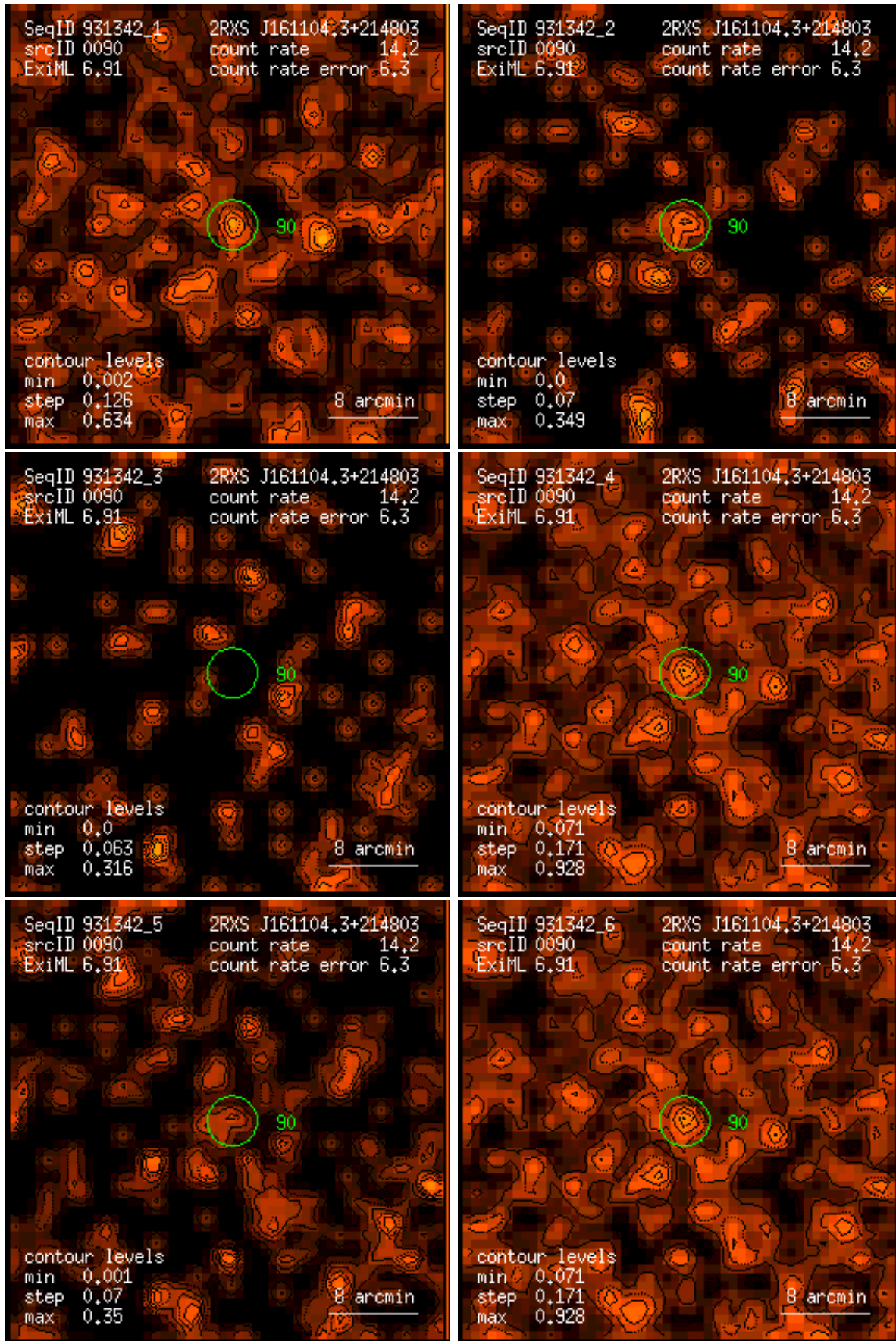
Figure 90: RASS 931342: detection 0090: band rate images, Gaussian filter: (1) PSPC channels 11 – 41, (2) 52 – 90, (3) 91 – 201, (4) 11 – 235, (5) 52 – 201, (6) 11 – 201. Broad band rates in counts/ks. Band rate contour levels in counts/ks/arcmin 2 .
