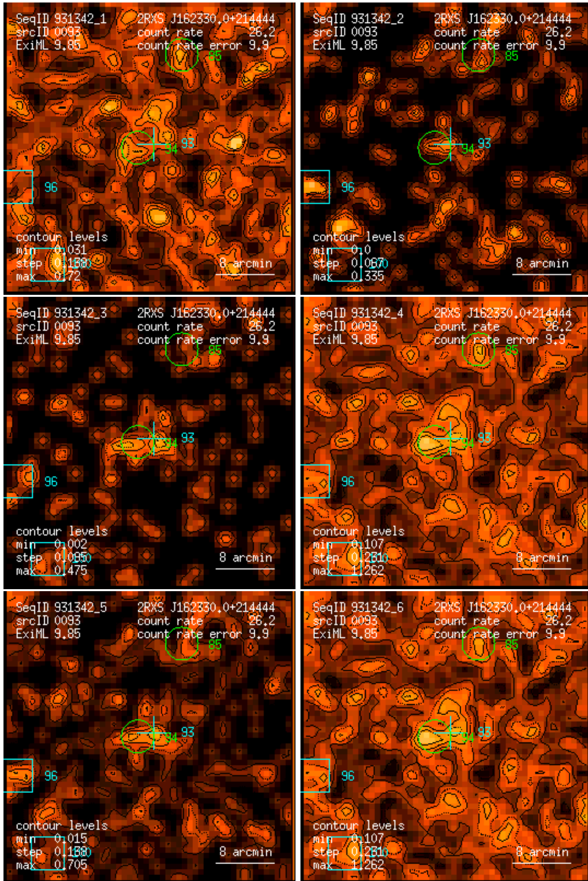
Figure 93: RASS 931342: detection 0093: band rate images, Gaussian filter: (1) PSPC channels 11 – 41, (2) 52 – 90, (3) 91 – 201, (4) 11 – 235, (5) 52 – 201, (6) 11 – 201. Broad band rates in counts/ks. Band rate contour levels in counts/ks/arcmin 2 .
