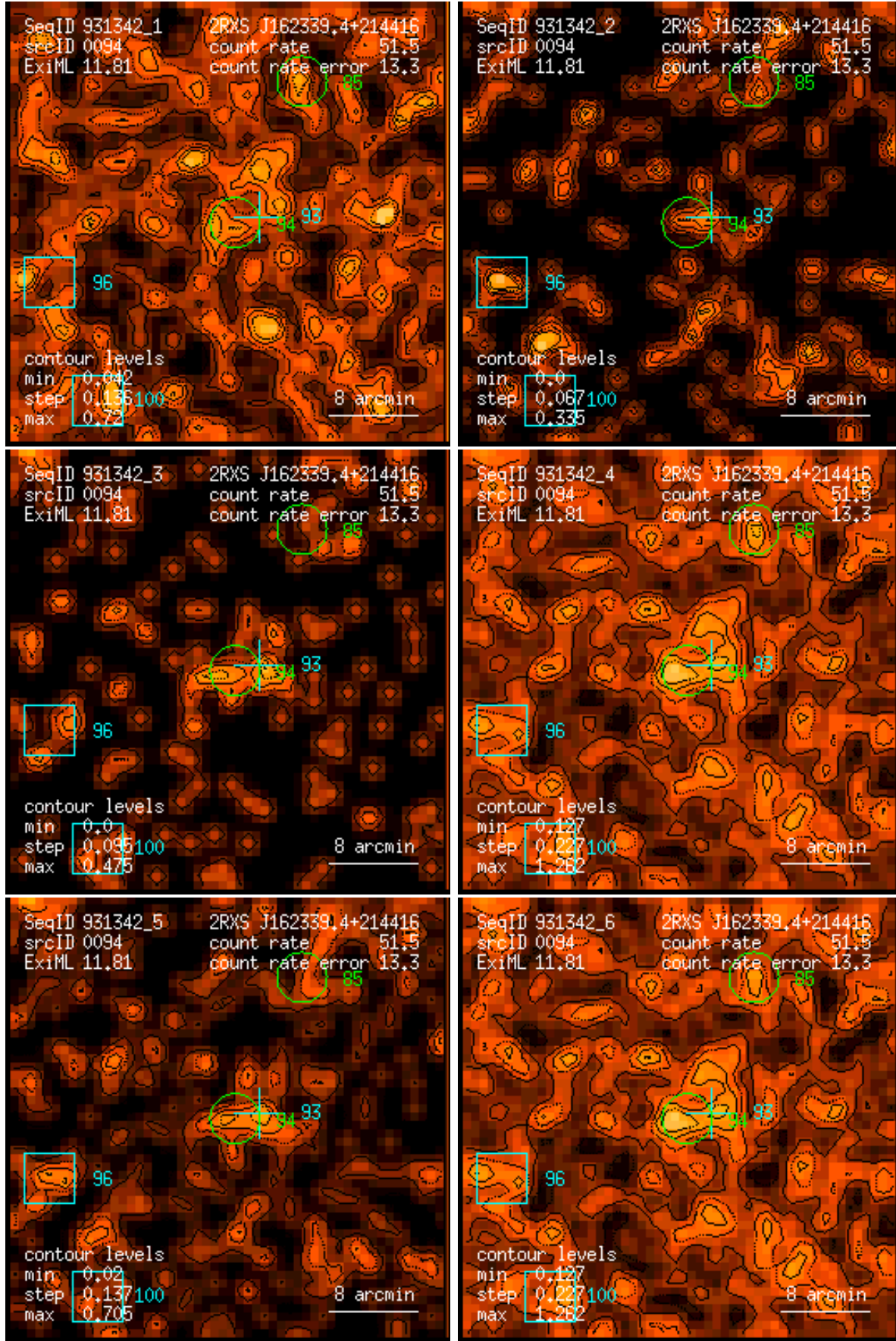
Figure 94: RASS 931342: detection 0094: band rate images, Gaussian filter: (1) PSPC channels 11 – 41, (2) 52 – 90, (3) 91 – 201, (4) 11 – 235, (5) 52 – 201, (6) 11 – 201. Broad band rates in counts/ks. Band rate contour levels in counts/ks/arcmin 2 .
