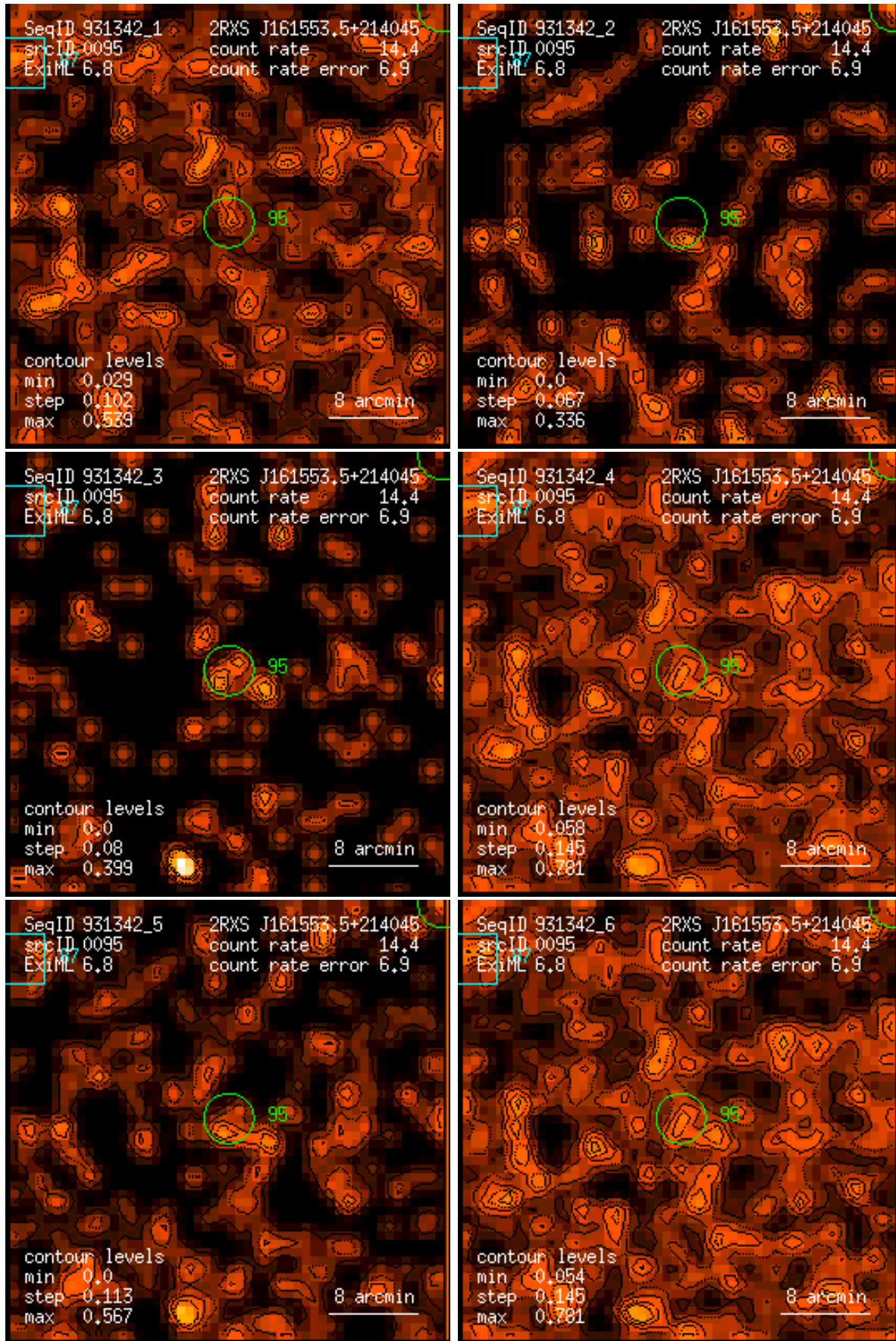
Figure 95: RASS 931342: detection 0095: band rate images, Gaussian filter: (1) PSPC channels 11 – 41, (2) 52 – 90, (3) 91 – 201, (4) 11 – 235, (5) 52 – 201, (6) 11 – 201. Broad band rates in counts/ks. Band rate contour levels in counts/ks/arcmin 2 .
