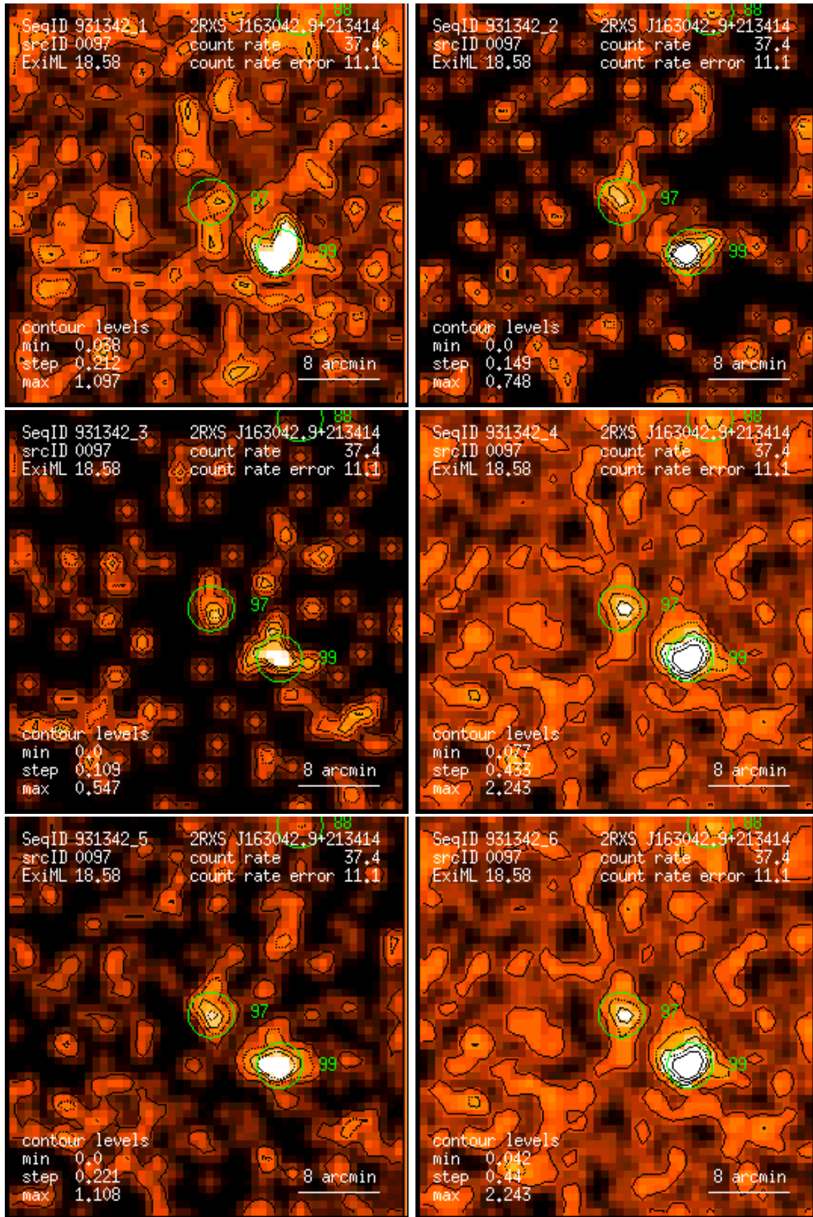
Figure 97: RASS 931342: detection 0097: band rate images, Gaussian filter: (1) PSPC channels 11 – 41, (2) 52 – 90, (3) 91 – 201, (4) 11 – 235, (5) 52 – 201, (6) 11 – 201. Broad band rates in counts/ks. Band rate contour levels in counts/ks/arcmin 2 .
