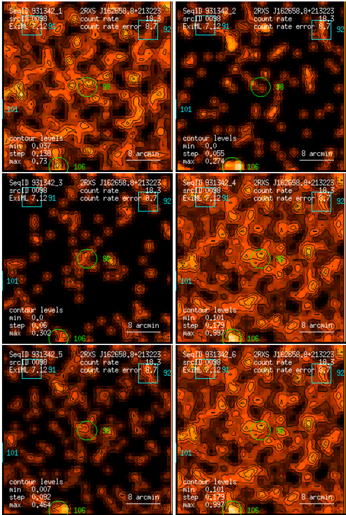
Figure 98: RASS 931342: detection 0098: band rate images, Gaussian filter: (1) PSPC channels 11 – 41, (2) 52 – 90, (3) 91 – 201, (4) 11 – 235, (5) 52 – 201, (6) 11 – 201. Broad band rates in counts/ks. Band rate contour levels in counts/ks/arcmin 2 .
