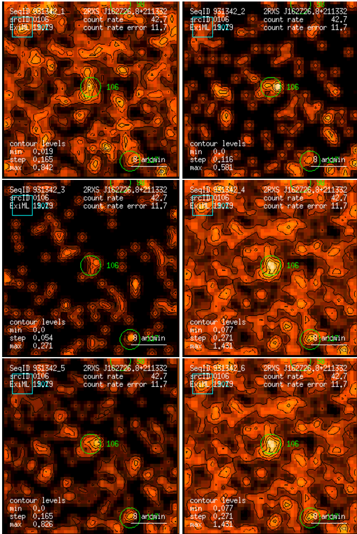
Figure 106: RASS 931342: detection 0106: band rate images, Gaussian filter: (1) PSPC channels 11 – 41, (2) 52 – 90, (3) 91 – 201, (4) 11 – 235, (5) 52 – 201, (6) 11 – 201. Broad band rates in counts/ks. Band rate contour levels in counts/ks/arcmin 2 .
