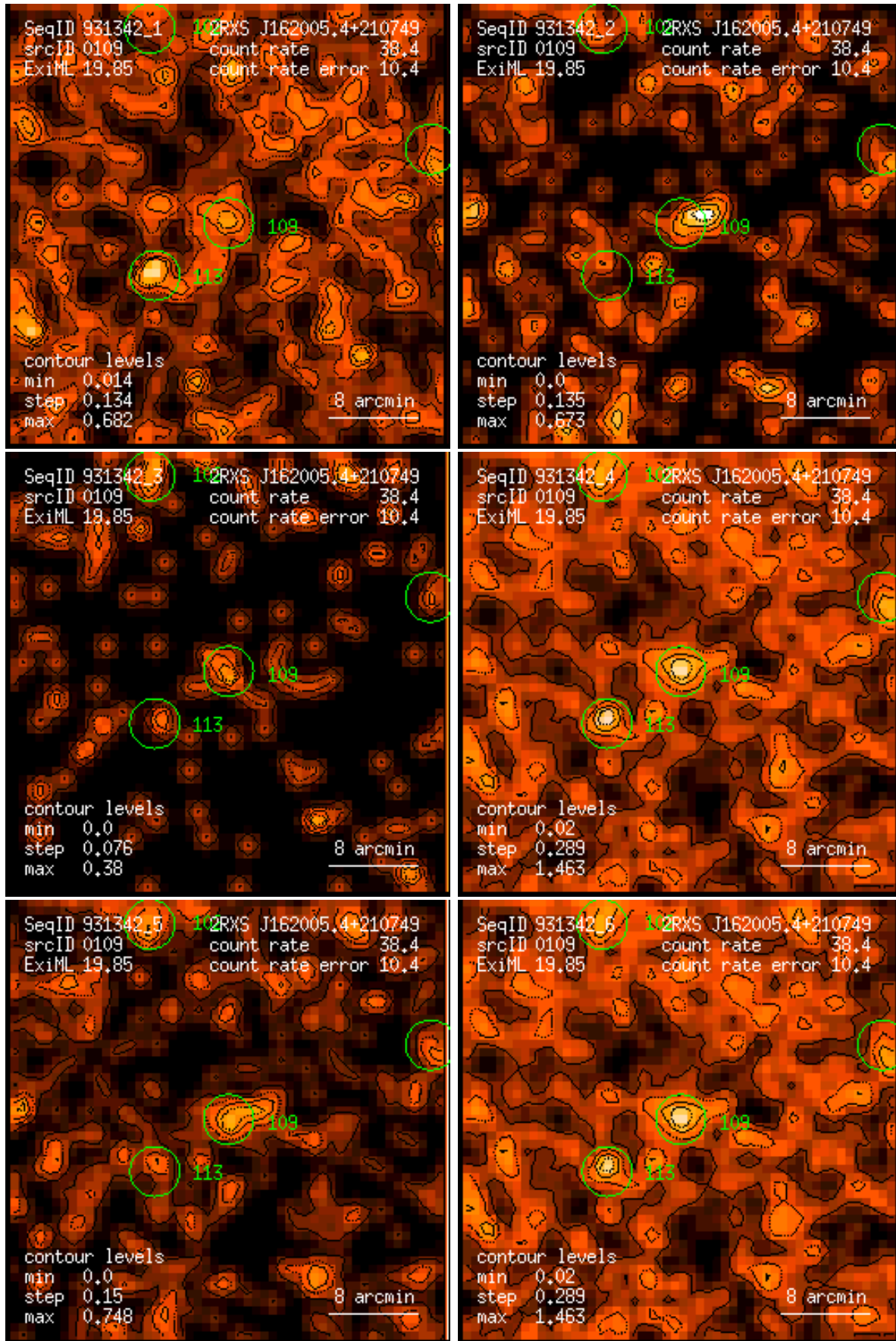
Figure 109: RASS 931342: detection 0109: band rate images, Gaussian filter: (1) PSPC channels 11 – 41, (2) 52 – 90, (3) 91 – 201, (4) 11 – 235, (5) 52 – 201, (6) 11 – 201. Broad band rates in counts/ks. Band rate contour levels in counts/ks/arcmin 2 .
