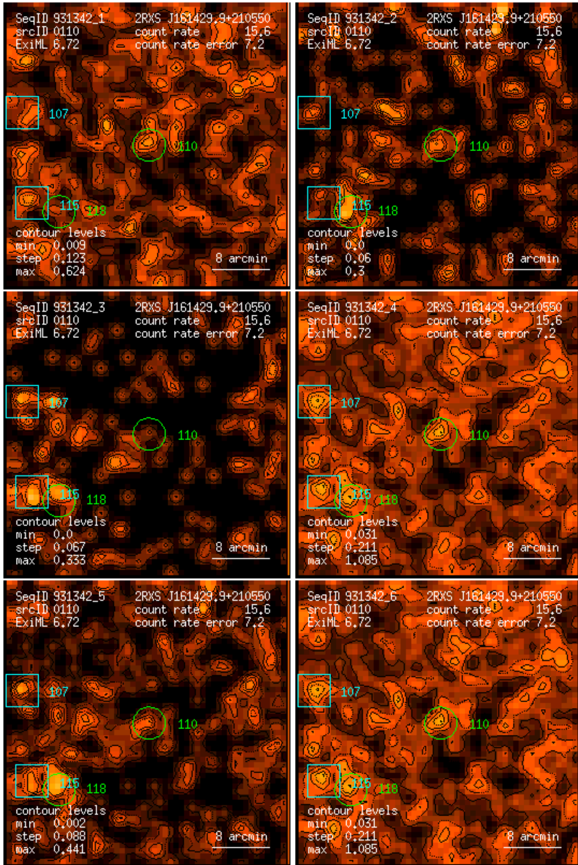
Figure 110: RASS 931342: detection 0110: band rate images, Gaussian filter: (1) PSPC channels 11 – 41, (2) 52 – 90, (3) 91 – 201, (4) 11 – 235, (5) 52 – 201, (6) 11 – 201. Broad band rates in counts/ks. Band rate contour levels in counts/ks/arcmin 2 .
