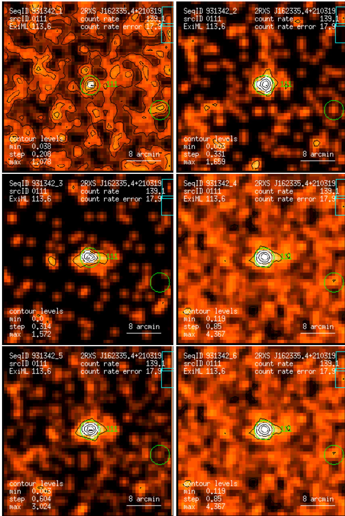
Figure 111: RASS 931342: detection 0111: band rate images, Gaussian filter: (1) PSPC channels 11 – 41, (2) 52 – 90, (3) 91 – 201, (4) 11 – 235, (5) 52 – 201, (6) 11 – 201. Broad band rates in counts/ks. Band rate contour levels in counts/ks/arcmin 2 .
