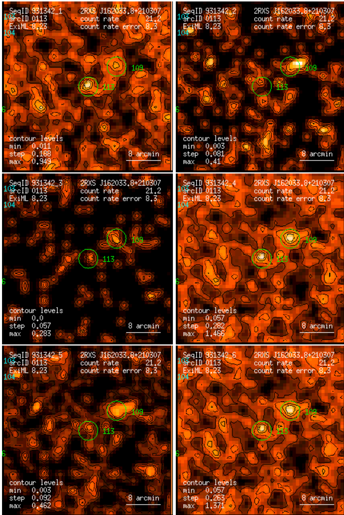
Figure 113: RASS 931342: detection 0113: band rate images, Gaussian filter: (1) PSPC channels 11 – 41, (2) 52 – 90, (3) 91 – 201, (4) 11 – 235, (5) 52 – 201, (6) 11 – 201. Broad band rates in counts/ks. Band rate contour levels in counts/ks/arcmin 2 .
