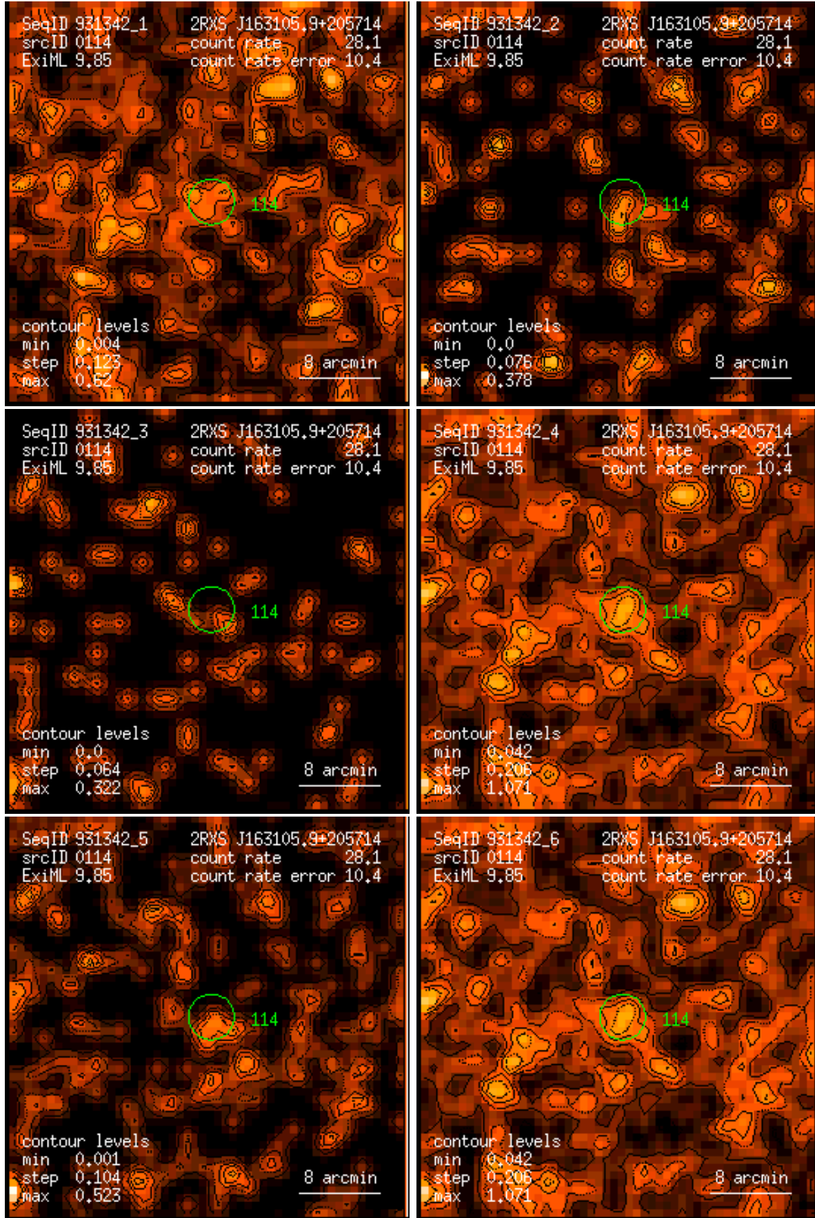
Figure 114: RASS 931342: detection 0114: band rate images, Gaussian filter: (1) PSPC channels 11 – 41, (2) 52 – 90, (3) 91 – 201, (4) 11 – 235, (5) 52 – 201, (6) 11 – 201. Broad band rates in counts/ks. Band rate contour levels in counts/ks/arcmin 2 .
