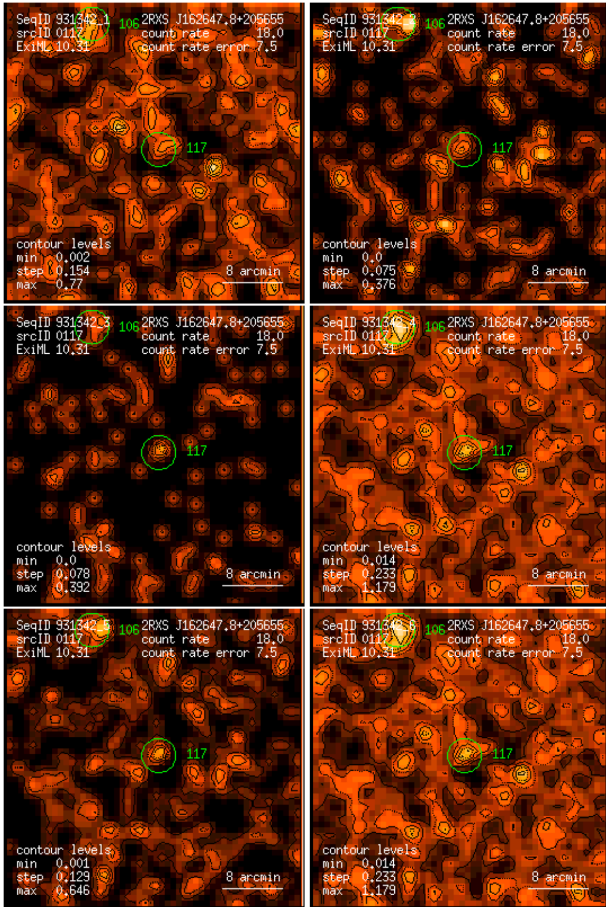
Figure 117: RASS 931342: detection 0117: band rate images, Gaussian filter: (1) PSPC channels 11 – 41, (2) 52 – 90, (3) 91 – 201, (4) 11 – 235, (5) 52 – 201, (6) 11 – 201. Broad band rates in counts/ks. Band rate contour levels in counts/ks/arcmin 2 .
