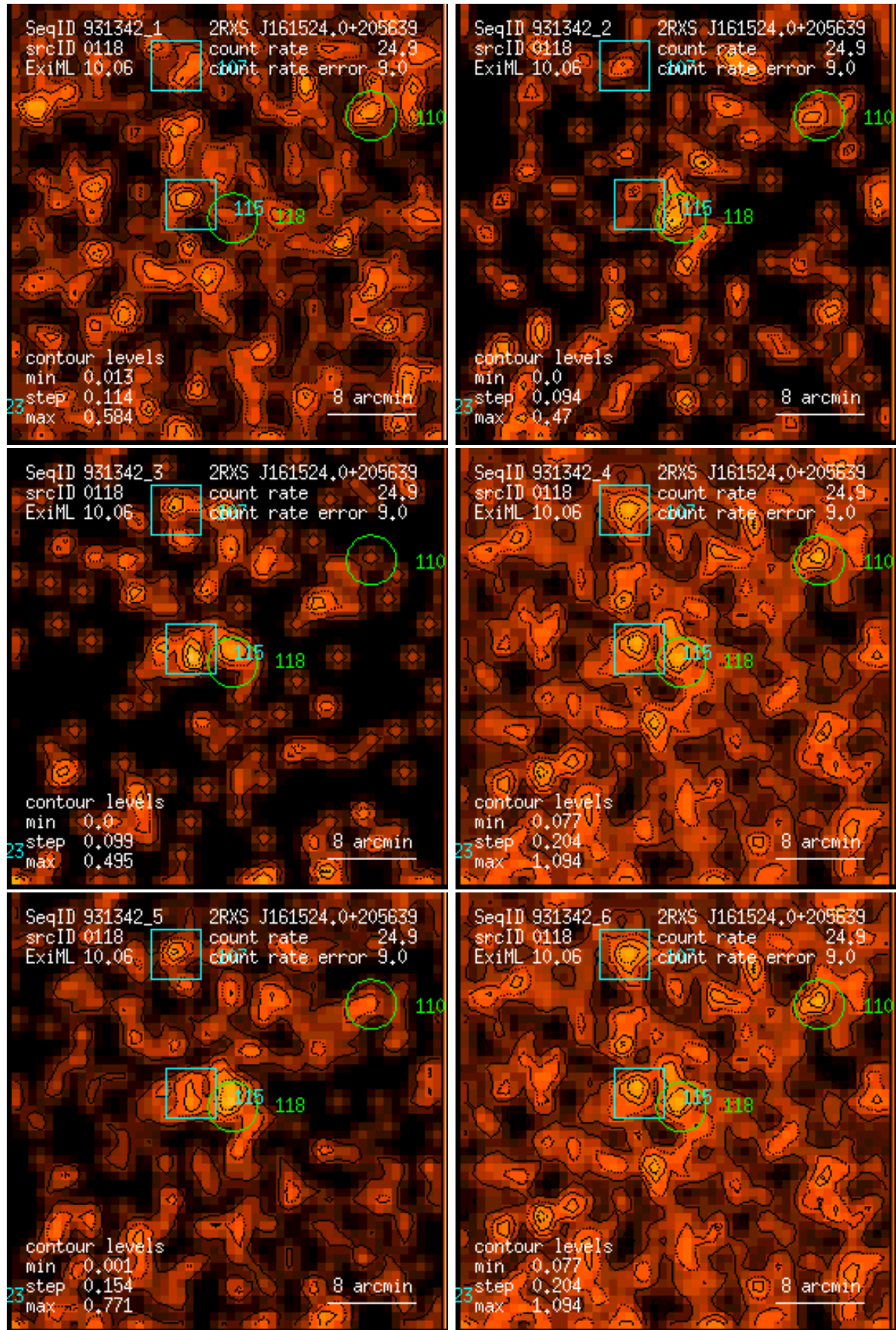
Figure 118: RASS 931342: detection 0118: band rate images, Gaussian filter: (1) PSPC channels 11 – 41, (2) 52 – 90, (3) 91 – 201, (4) 11 – 235, (5) 52 – 201, (6) 11 – 201. Broad band rates in counts/ks. Band rate contour levels in counts/ks/arcmin 2 .
