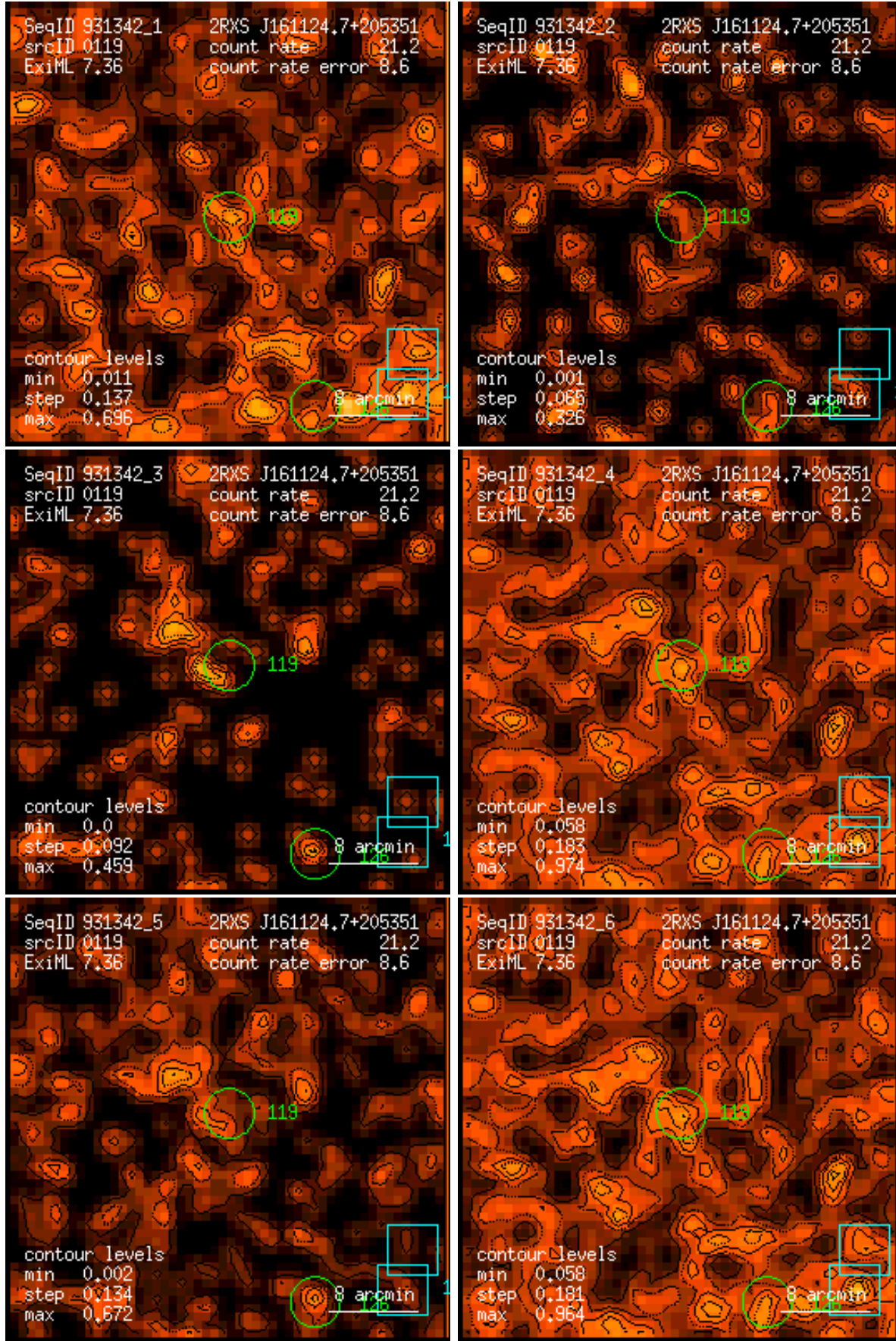
Figure 119: RASS 931342: detection 0119: band rate images, Gaussian filter: (1) PSPC channels 11 – 41, (2) 52 – 90, (3) 91 – 201, (4) 11 – 235, (5) 52 – 201, (6) 11 – 201. Broad band rates in counts/ks. Band rate contour levels in counts/ks/arcmin 2 .
