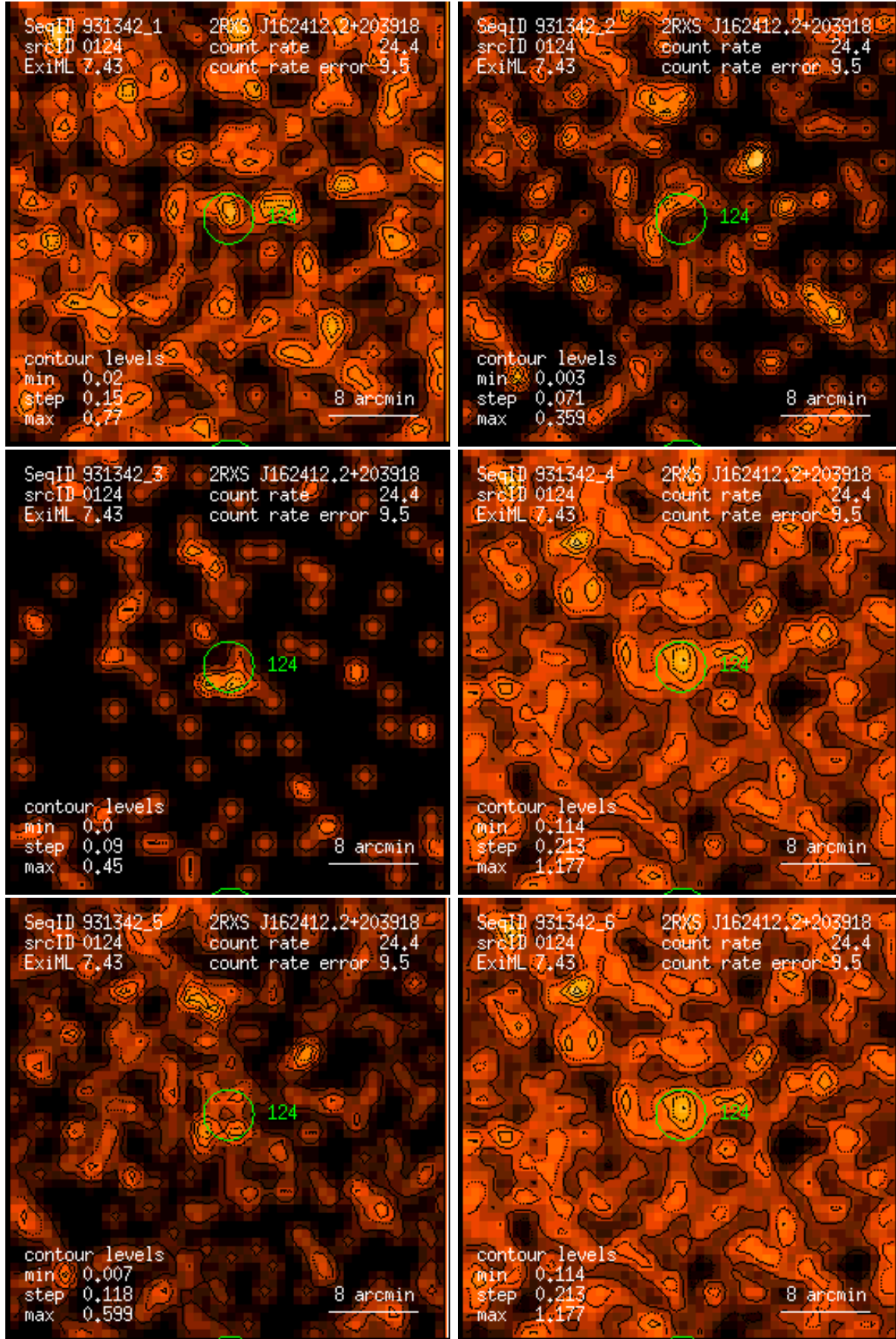
Figure 124: RASS 931342: detection 0124: band rate images, Gaussian filter: (1) PSPC channels 11 – 41, (2) 52 – 90, (3) 91 – 201, (4) 11 – 235, (5) 52 – 201, (6) 11 – 201. Broad band rates in counts/ks. Band rate contour levels in counts/ks/arcmin 2 .
