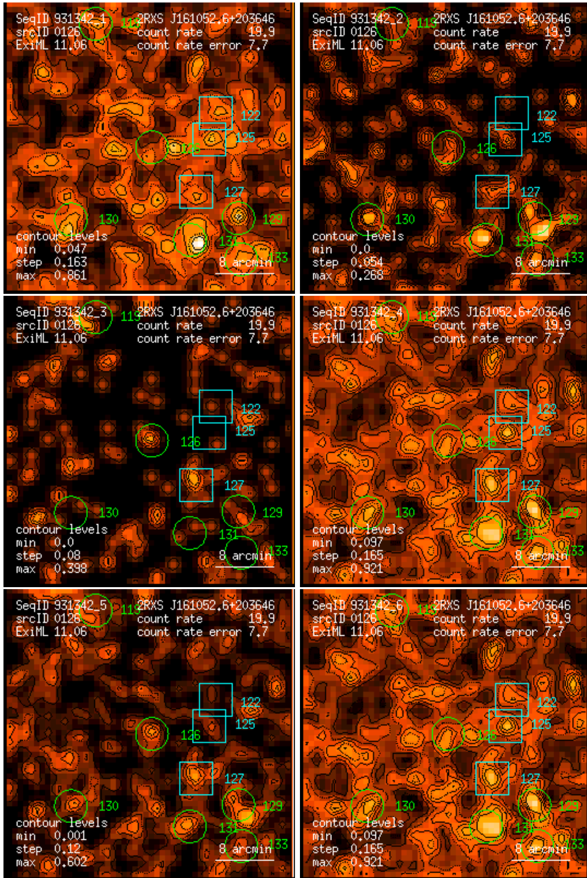
Figure 126: RASS 931342: detection 0126: band rate images, Gaussian filter: (1) PSPC channels 11 – 41, (2) 52 – 90, (3) 91 – 201, (4) 11 – 235, (5) 52 – 201, (6) 11 – 201. Broad band rates in counts/ks. Band rate contour levels in counts/ks/arcmin 2 .
