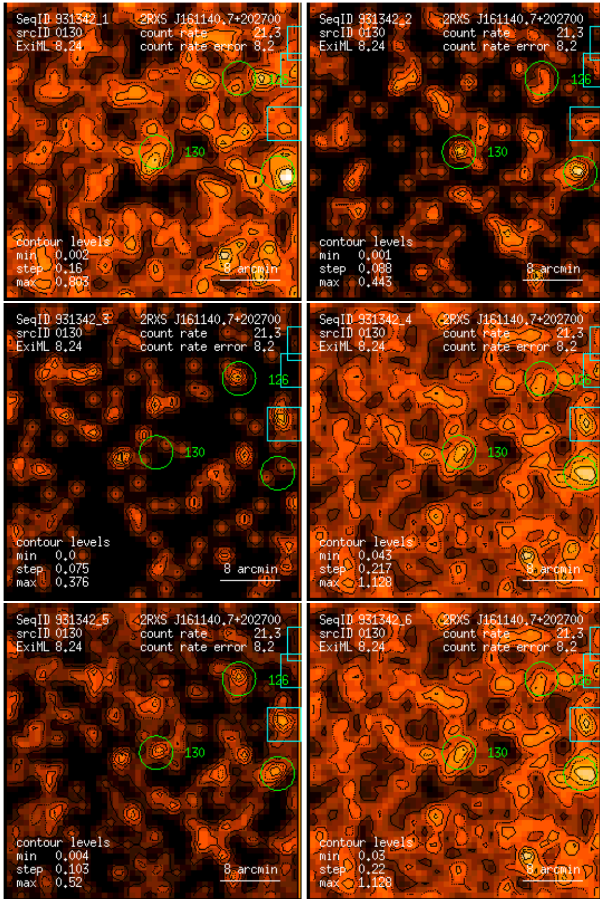
Figure 130: RASS 931342: detection 0130: band rate images, Gaussian filter: (1) PSPC channels 11 – 41, (2) 52 – 90, (3) 91 – 201, (4) 11 – 235, (5) 52 – 201, (6) 11 – 201. Broad band rates in counts/ks. Band rate contour levels in counts/ks/arcmin 2 .
