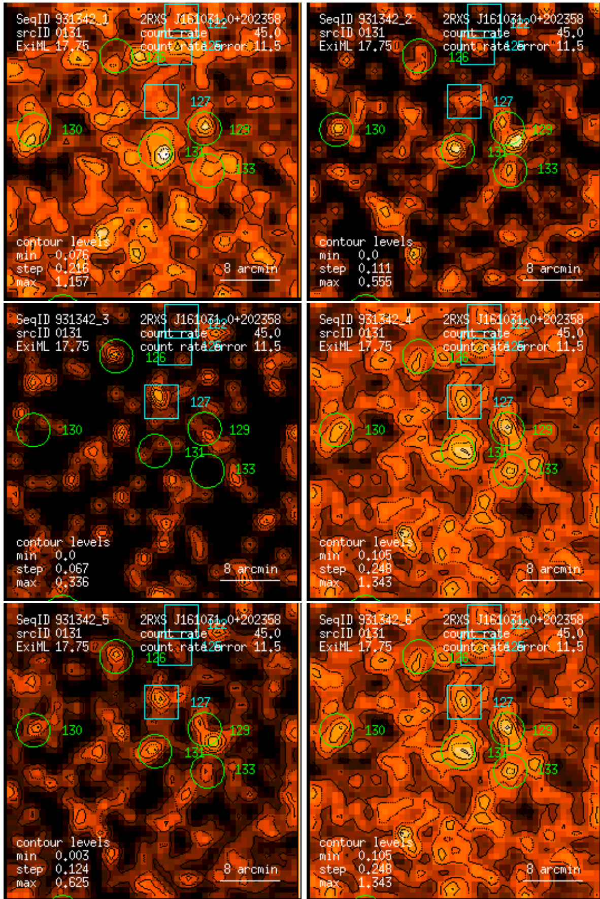
Figure 131: RASS 931342: detection 0131: band rate images, Gaussian filter: (1) PSPC channels 11 – 41, (2) 52 – 90, (3) 91 – 201, (4) 11 – 235, (5) 52 – 201, (6) 11 – 201. Broad band rates in counts/ks. Band rate contour levels in counts/ks/arcmin 2 .
