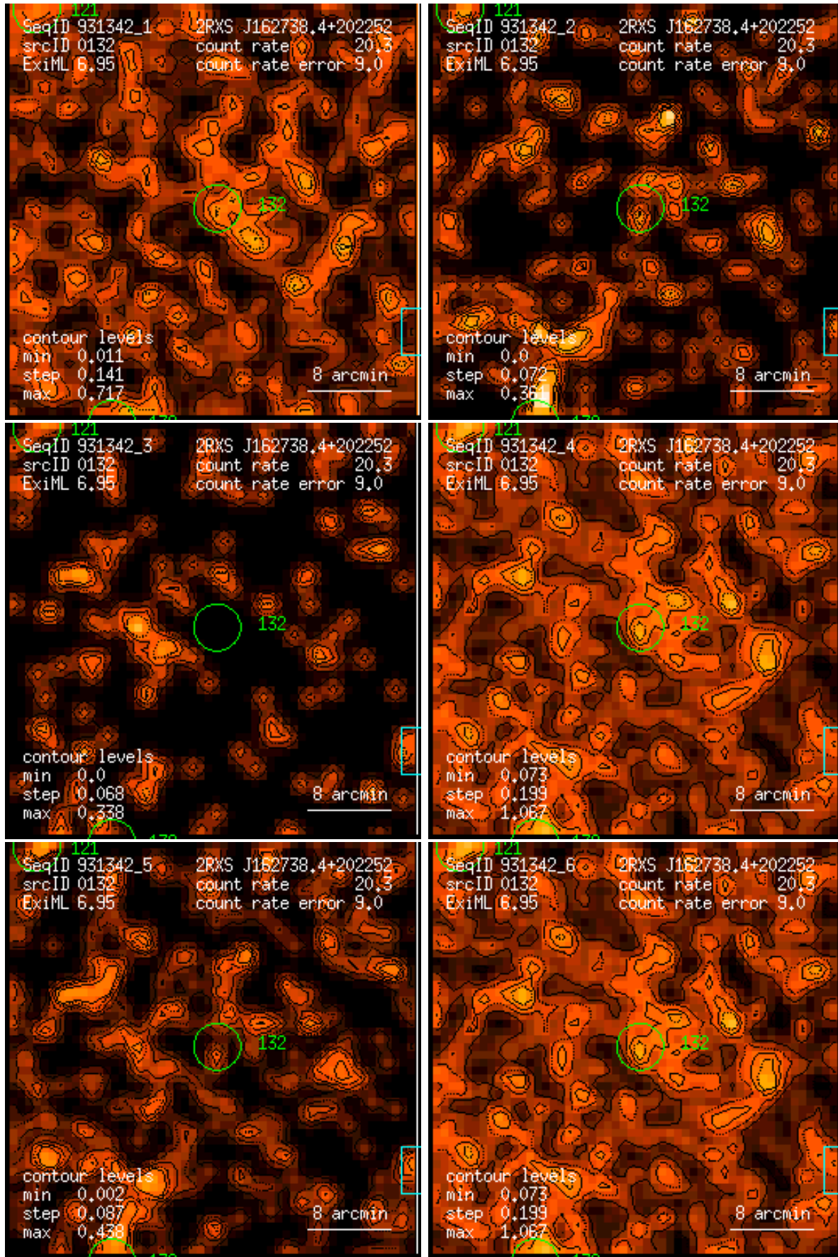
Figure 132: RASS 931342: detection 0132: band rate images, Gaussian filter: (1) PSPC channels 11 – 41, (2) 52 – 90, (3) 91 – 201, (4) 11 – 235, (5) 52 – 201, (6) 11 – 201. Broad band rates in counts/ks. Band rate contour levels in counts/ks/arcmin 2 .
