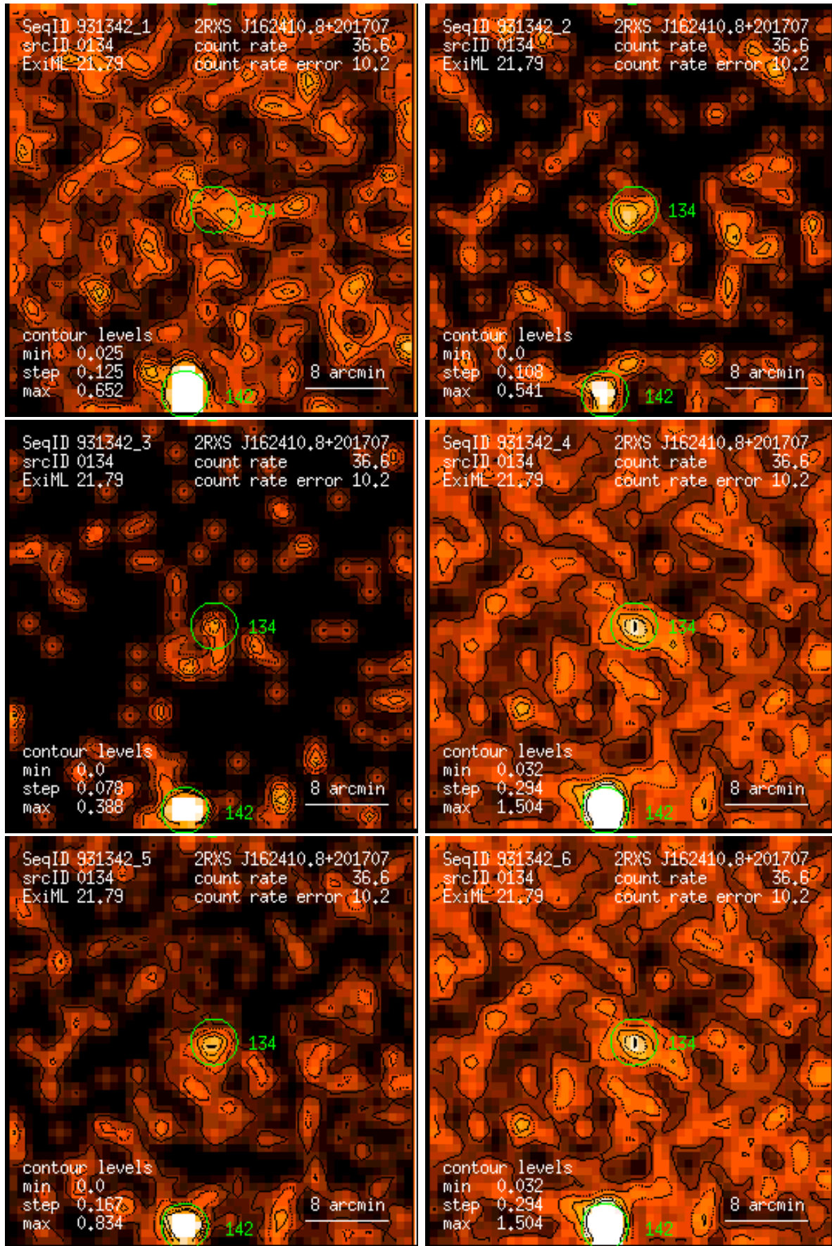
Figure 134: RASS 931342: detection 0134: band rate images, Gaussian filter: (1) PSPC channels 11 – 41, (2) 52 – 90, (3) 91 – 201, (4) 11 – 235, (5) 52 – 201, (6) 11 – 201. Broad band rates in counts/ks. Band rate contour levels in counts/ks/arcmin 2 .
