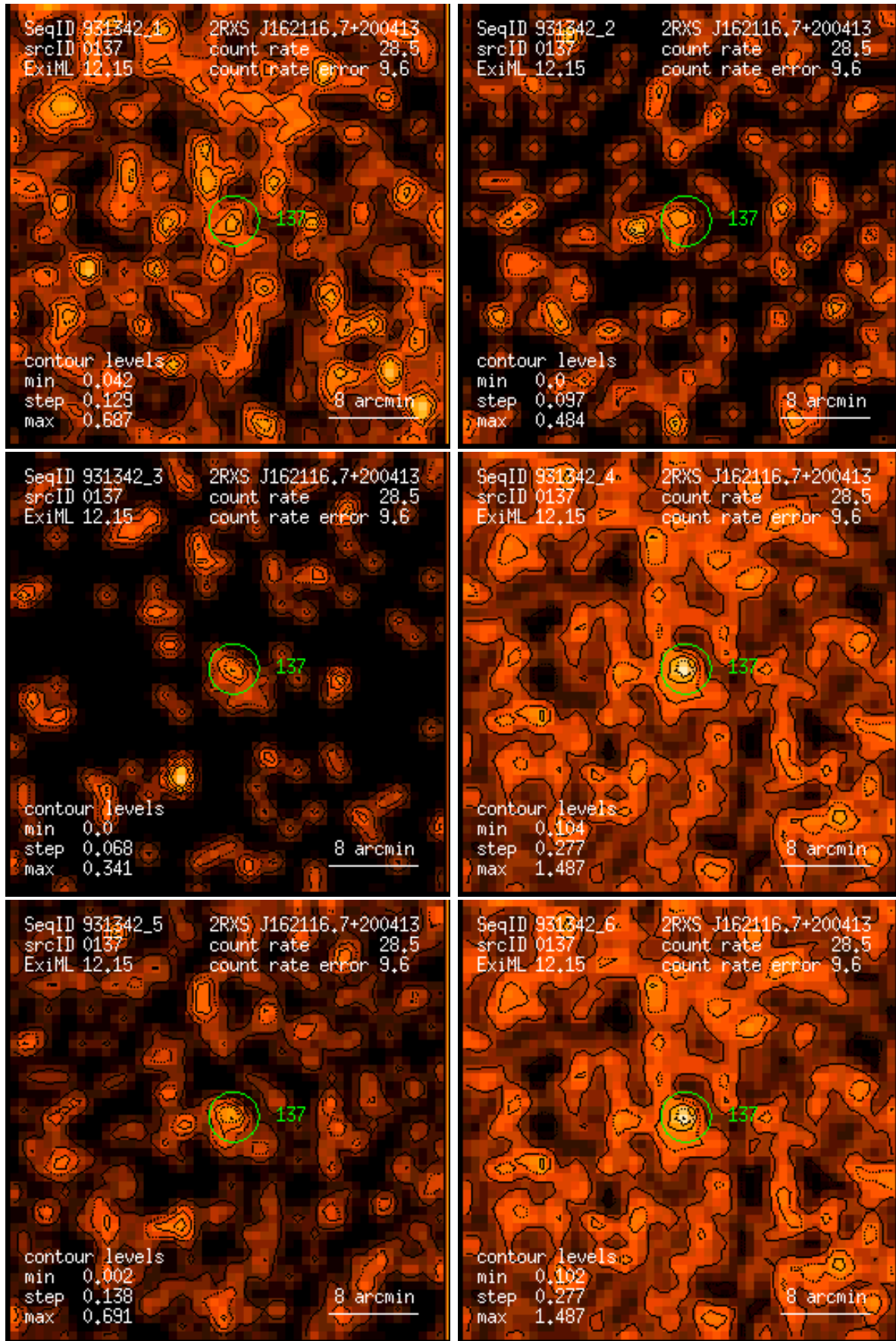
Figure 137: RASS 931342: detection 0137: band rate images, Gaussian filter: (1) PSPC channels 11 – 41, (2) 52 – 90, (3) 91 – 201, (4) 11 – 235, (5) 52 – 201, (6) 11 – 201. Broad band rates in counts/ks. Band rate contour levels in counts/ks/arcmin 2 .
