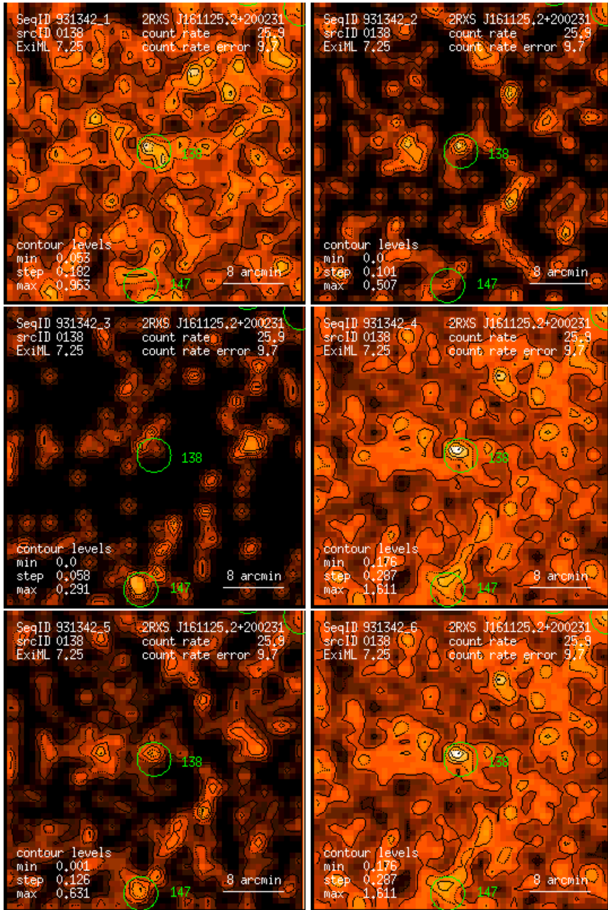
Figure 138: RASS 931342: detection 0138: band rate images, Gaussian filter: (1) PSPC channels 11 – 41, (2) 52 – 90, (3) 91 – 201, (4) 11 – 235, (5) 52 – 201, (6) 11 – 201. Broad band rates in counts/ks. Band rate contour levels in counts/ks/arcmin 2 .
