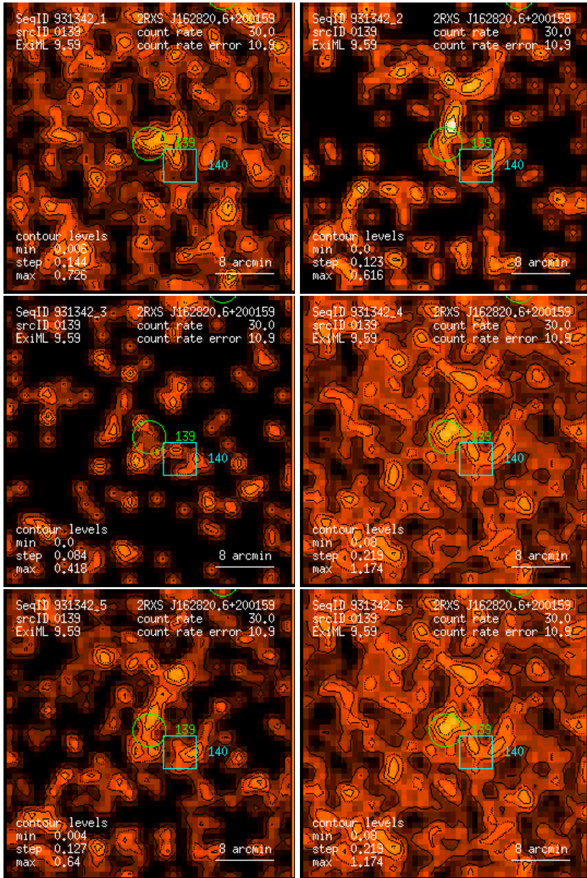
Figure 139: RASS 931342: detection 0139: band rate images, Gaussian filter: (1) PSPC channels 11 – 41, (2) 52 – 90, (3) 91 – 201, (4) 11 – 235, (5) 52 – 201, (6) 11 – 201. Broad band rates in counts/ks. Band rate contour levels in counts/ks/arcmin 2 .
