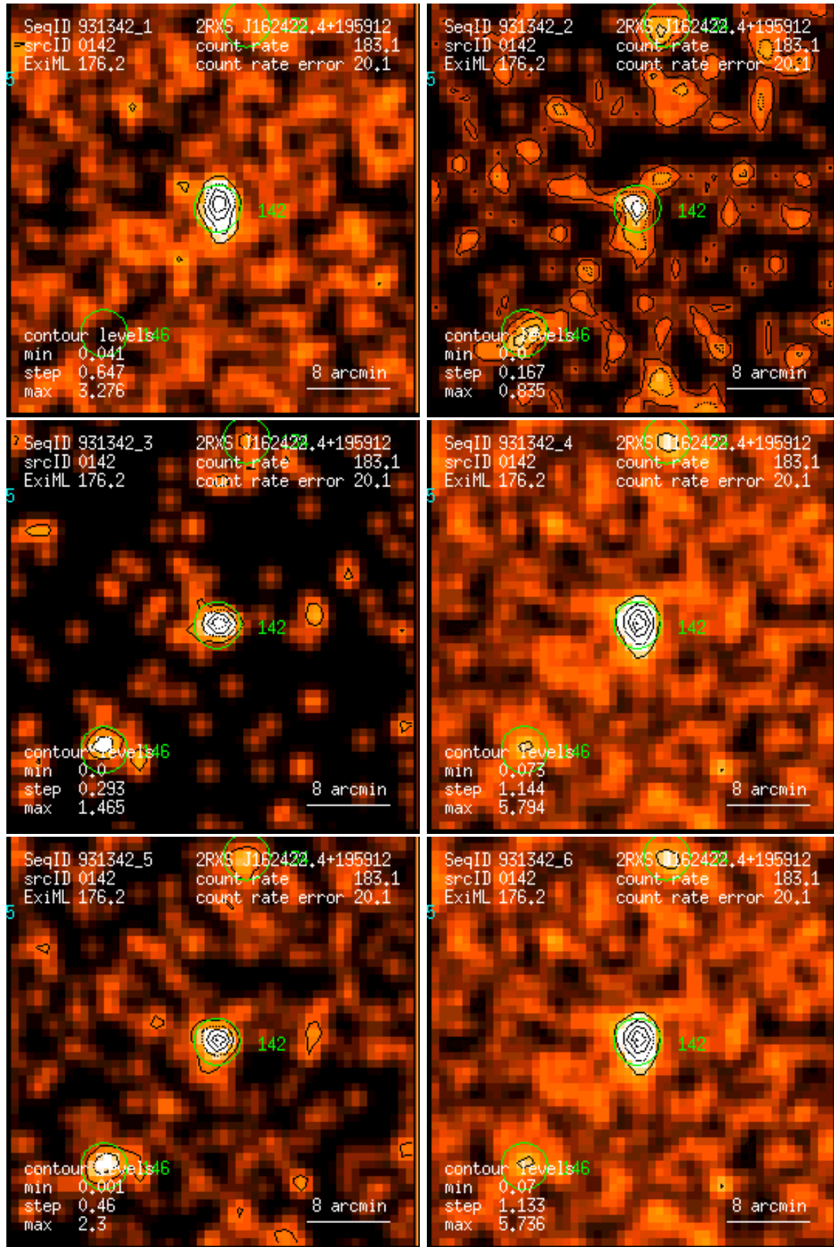
Figure 142: RASS 931342: detection 0142: band rate images, Gaussian filter: (1) PSPC channels 11 – 41, (2) 52 – 90, (3) 91 – 201, (4) 11 – 235, (5) 52 – 201, (6) 11 – 201. Broad band rates in counts/ks. Band rate contour levels in counts/ks/arcmin 2 .
