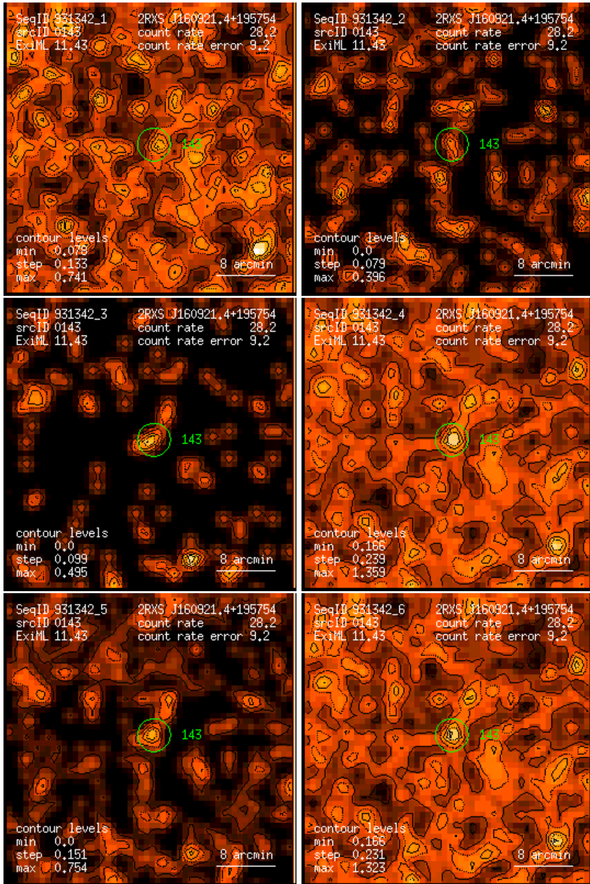
Figure 143: RASS 931342: detection 0143: band rate images, Gaussian filter: (1) PSPC channels 11 – 41, (2) 52 – 90, (3) 91 – 201, (4) 11 – 235, (5) 52 – 201, (6) 11 – 201. Broad band rates in counts/ks. Band rate contour levels in counts/ks/arcmin 2 .
