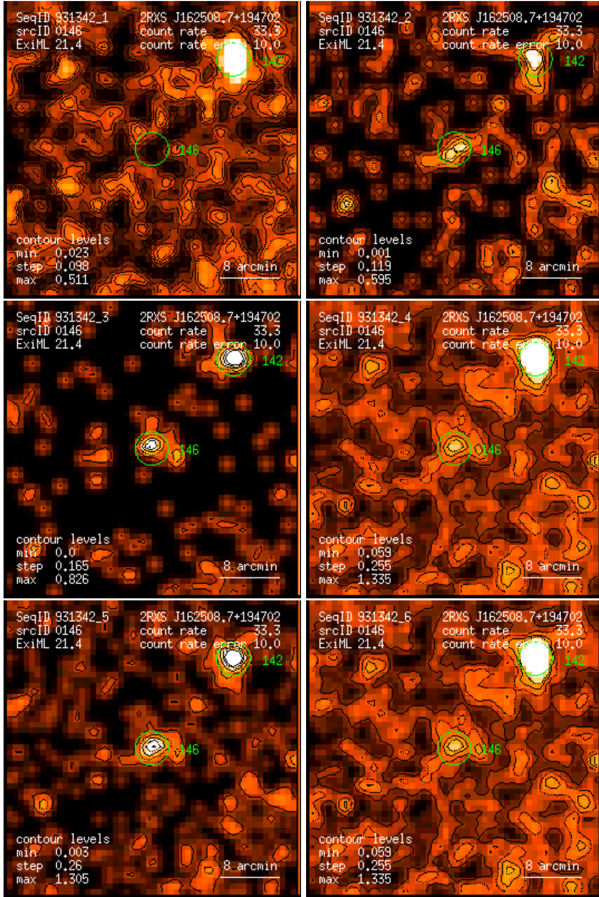
Figure 146: RASS 931342: detection 0146: band rate images, Gaussian filter: (1) PSPC channels 11 – 41, (2) 52 – 90, (3) 91 – 201, (4) 11 – 235, (5) 52 – 201, (6) 11 – 201. Broad band rates in counts/ks. Band rate contour levels in counts/ks/arcmin 2 .
