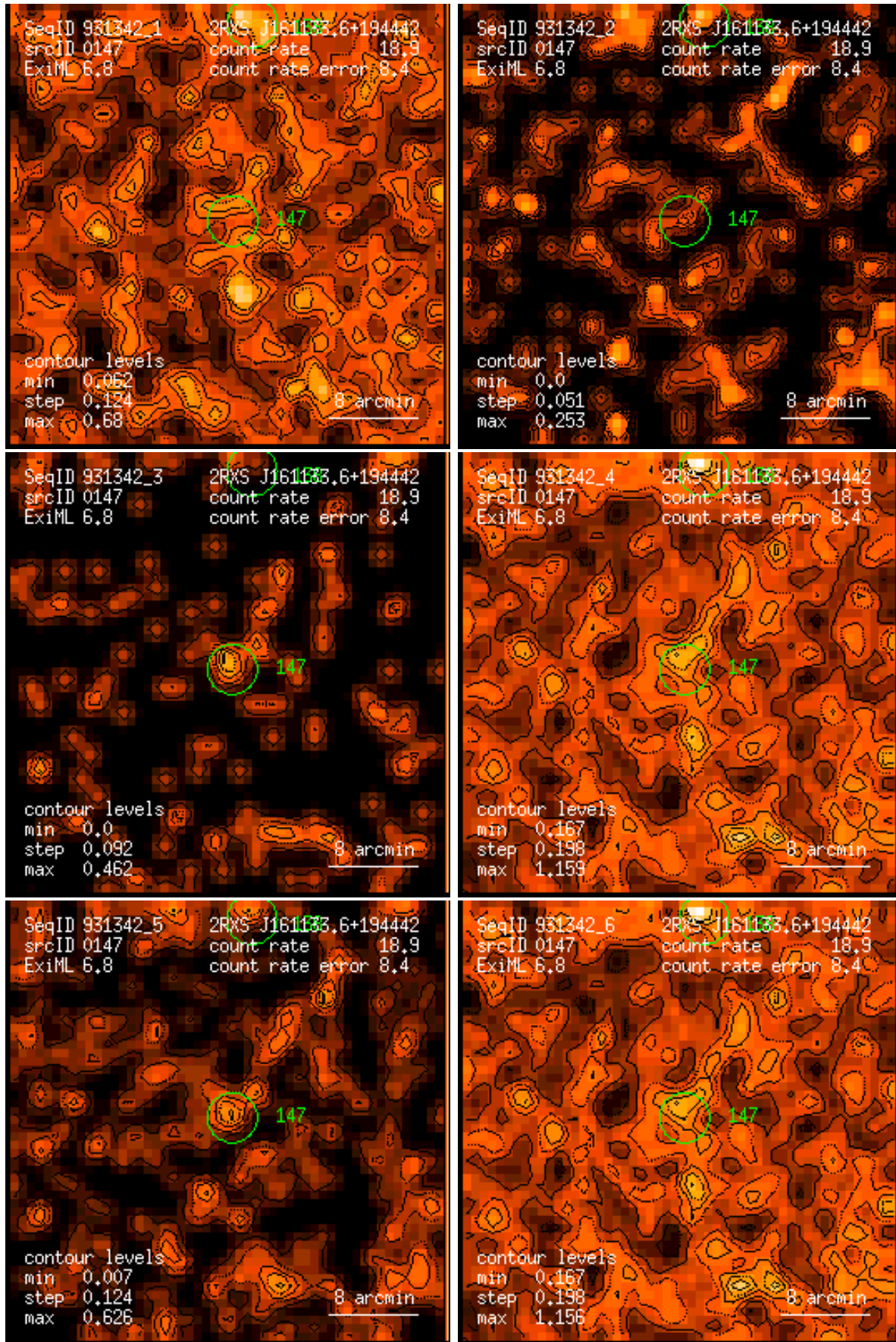
Figure 147: RASS 931342: detection 0147: band rate images, Gaussian filter: (1) PSPC channels 11 – 41, (2) 52 – 90, (3) 91 – 201, (4) 11 – 235, (5) 52 – 201, (6) 11 – 201. Broad band rates in counts/ks. Band rate contour levels in counts/ks/arcmin 2 .
