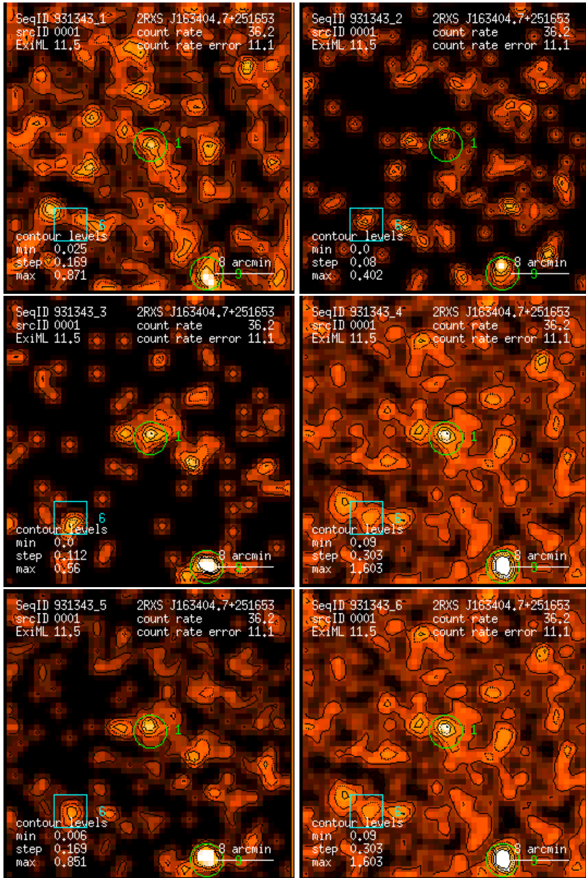
Figure 1: RASS 931343: detection 0001: band rate images, Gaussian filter: (1) PSPC channels 11 – 41, (2) 52 – 90, (3) 91 – 201, (4) 11 – 235, (5) 52 – 201, (6) 11 – 201. Broad band rates in counts/ks. Band rate contour levels in counts/ks/arcmin 2 .
