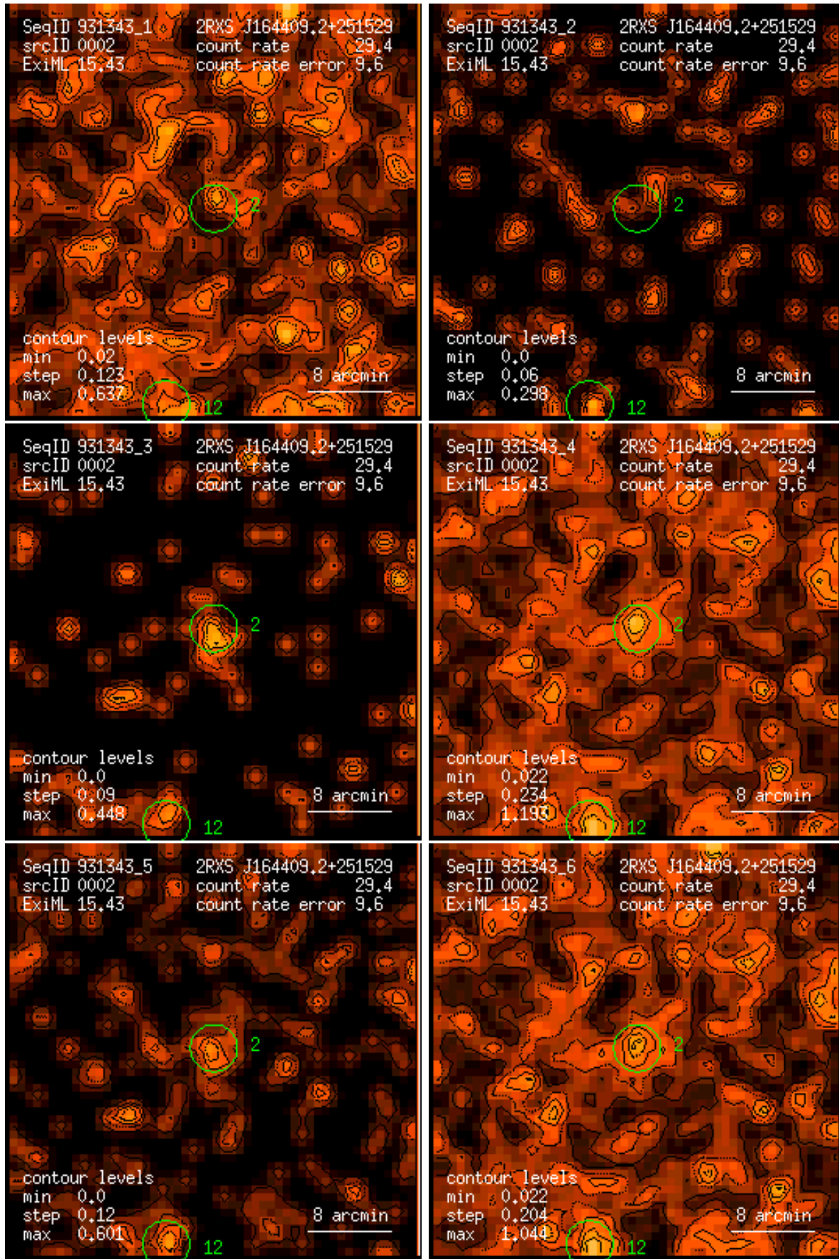
Figure 2: RASS 931343: detection 0002: band rate images, Gaussian filter: (1) PSPC channels 11 – 41, (2) 52 – 90, (3) 91 – 201, (4) 11 – 235, (5) 52 – 201, (6) 11 – 201. Broad band rates in counts/ks. Band rate contour levels in counts/ks/arcmin 2 .
