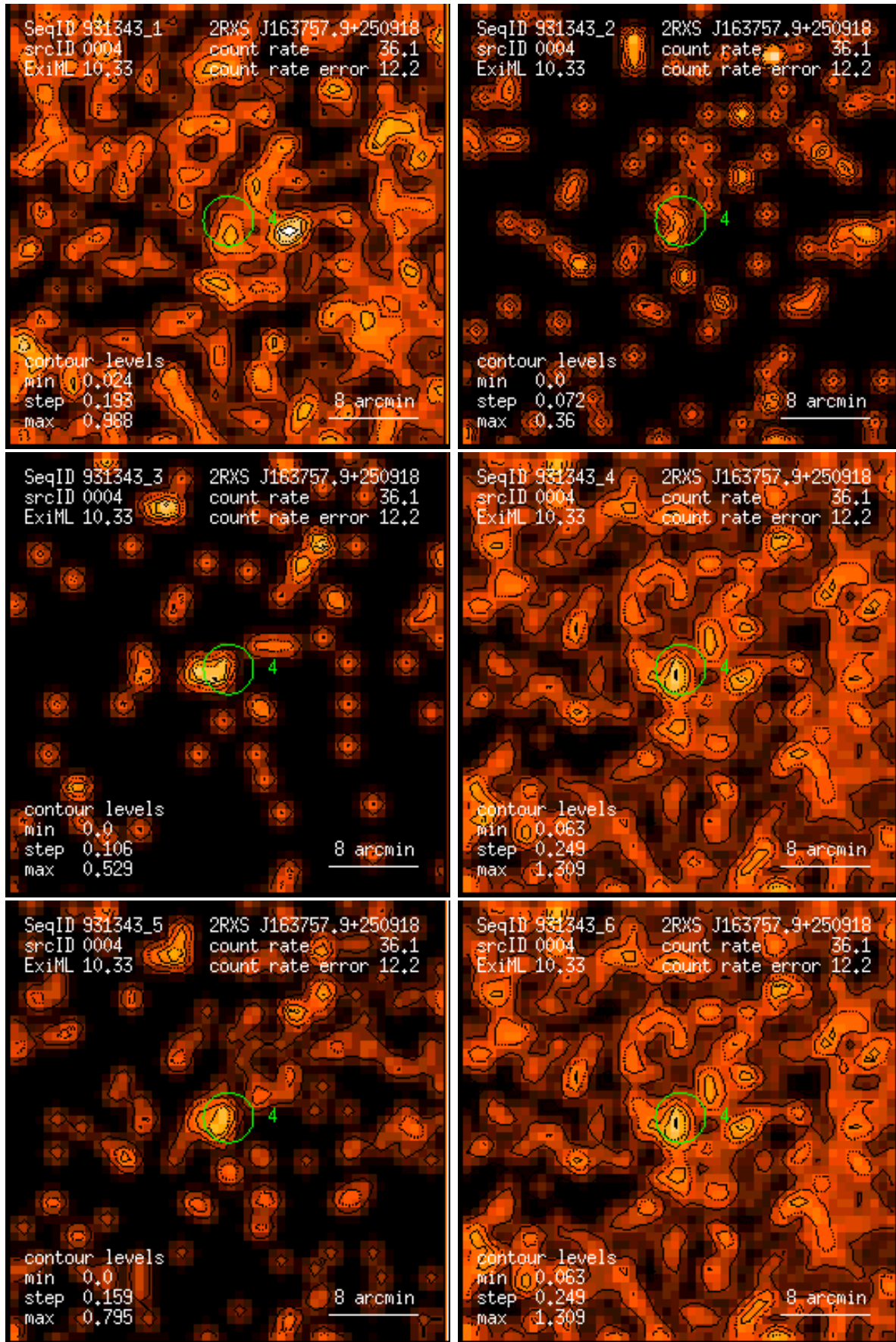
Figure 4: RASS 931343: detection 0004: band rate images, Gaussian filter: (1) PSPC channels 11 – 41, (2) 52 – 90, (3) 91 – 201, (4) 11 – 235, (5) 52 – 201, (6) 11 – 201. Broad band rates in counts/ks. Band rate contour levels in counts/ks/arcmin 2 .
