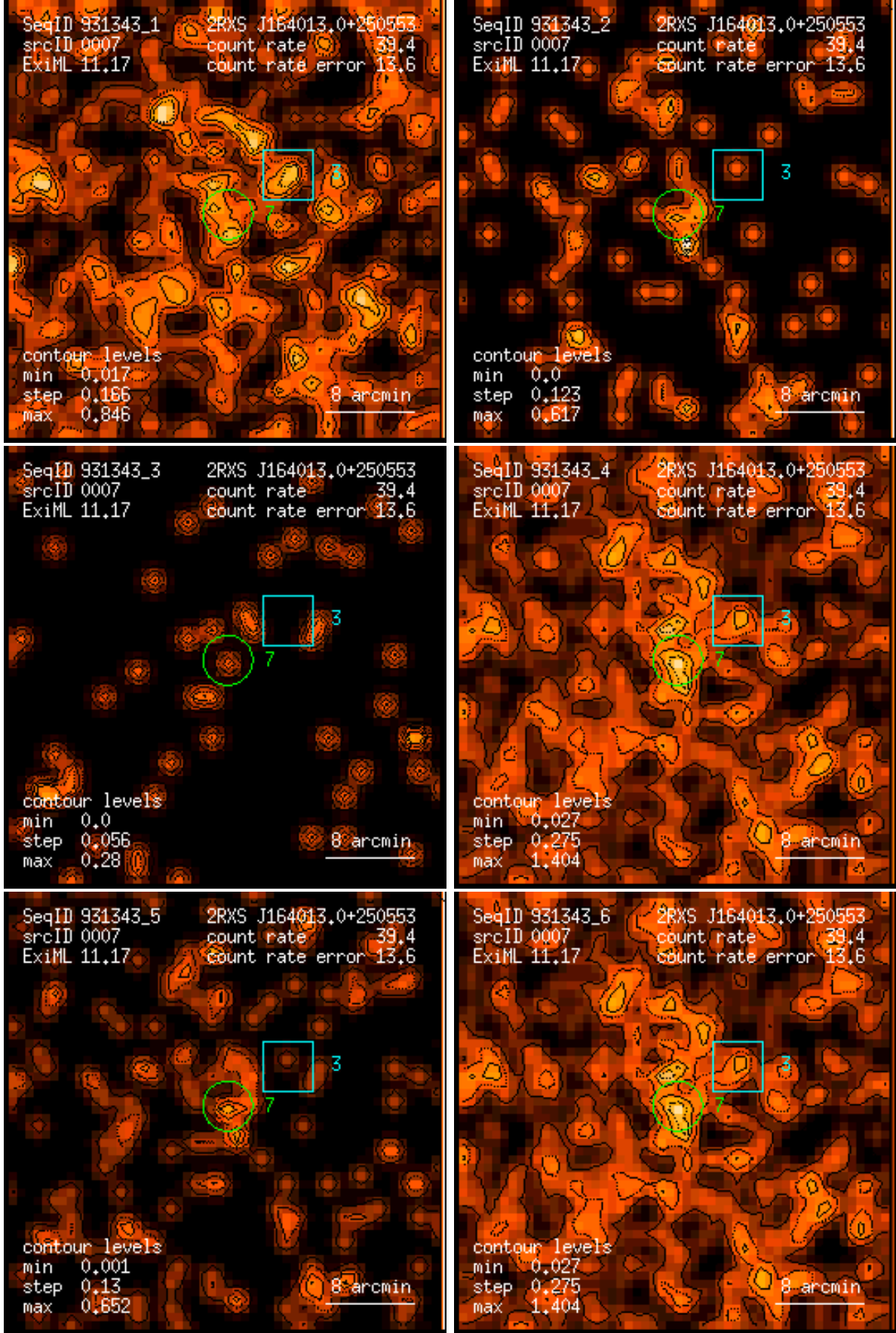
Figure 7: RASS 931343: detection 0007: band rate images, Gaussian filter: (1) PSPC channels 11 – 41, (2) 52 – 90, (3) 91 – 201, (4) 11 – 235, (5) 52 – 201, (6) 11 – 201. Broad band rates in counts/ks. Band rate contour levels in counts/ks/arcmin 2 .
