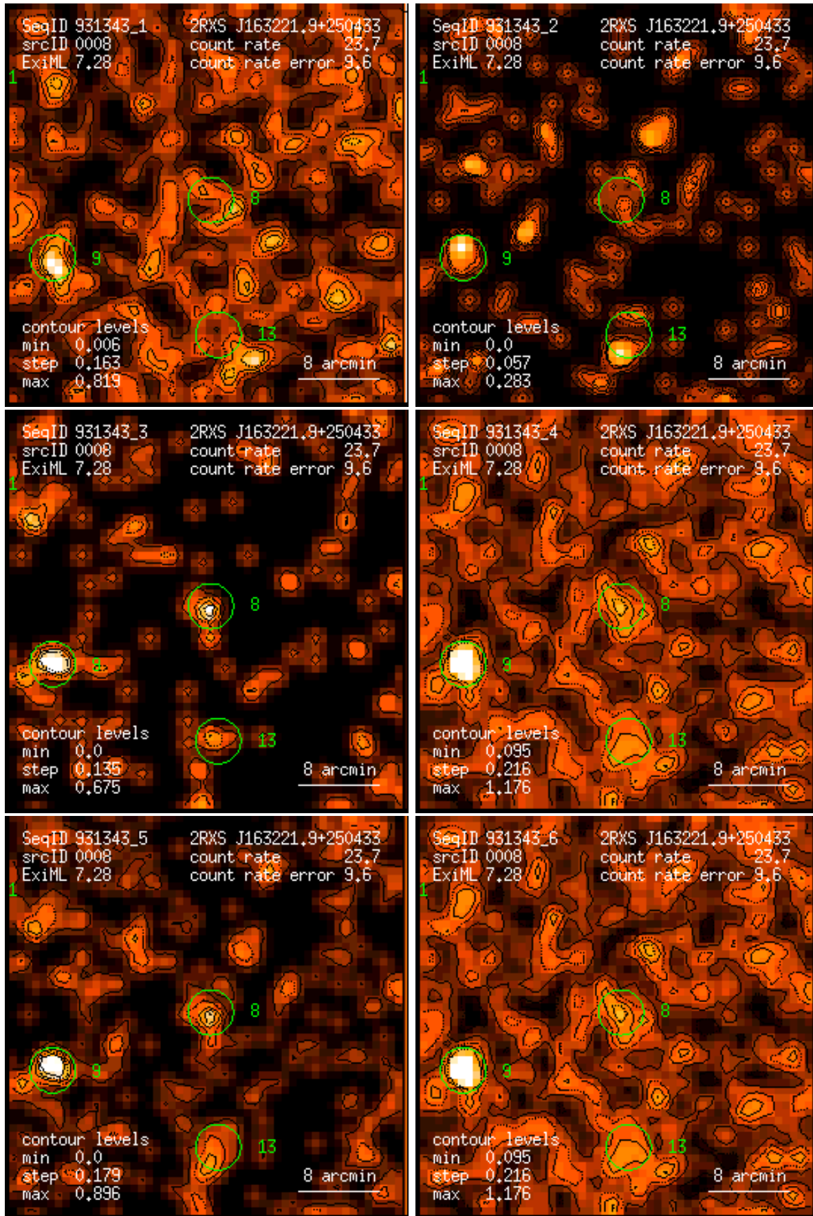
Figure 8: RASS 931343: detection 0008: band rate images, Gaussian filter: (1) PSPC channels 11 – 41, (2) 52 – 90, (3) 91 – 201, (4) 11 – 235, (5) 52 – 201, (6) 11 – 201. Broad band rates in counts/ks. Band rate contour levels in counts/ks/arcmin 2 .
