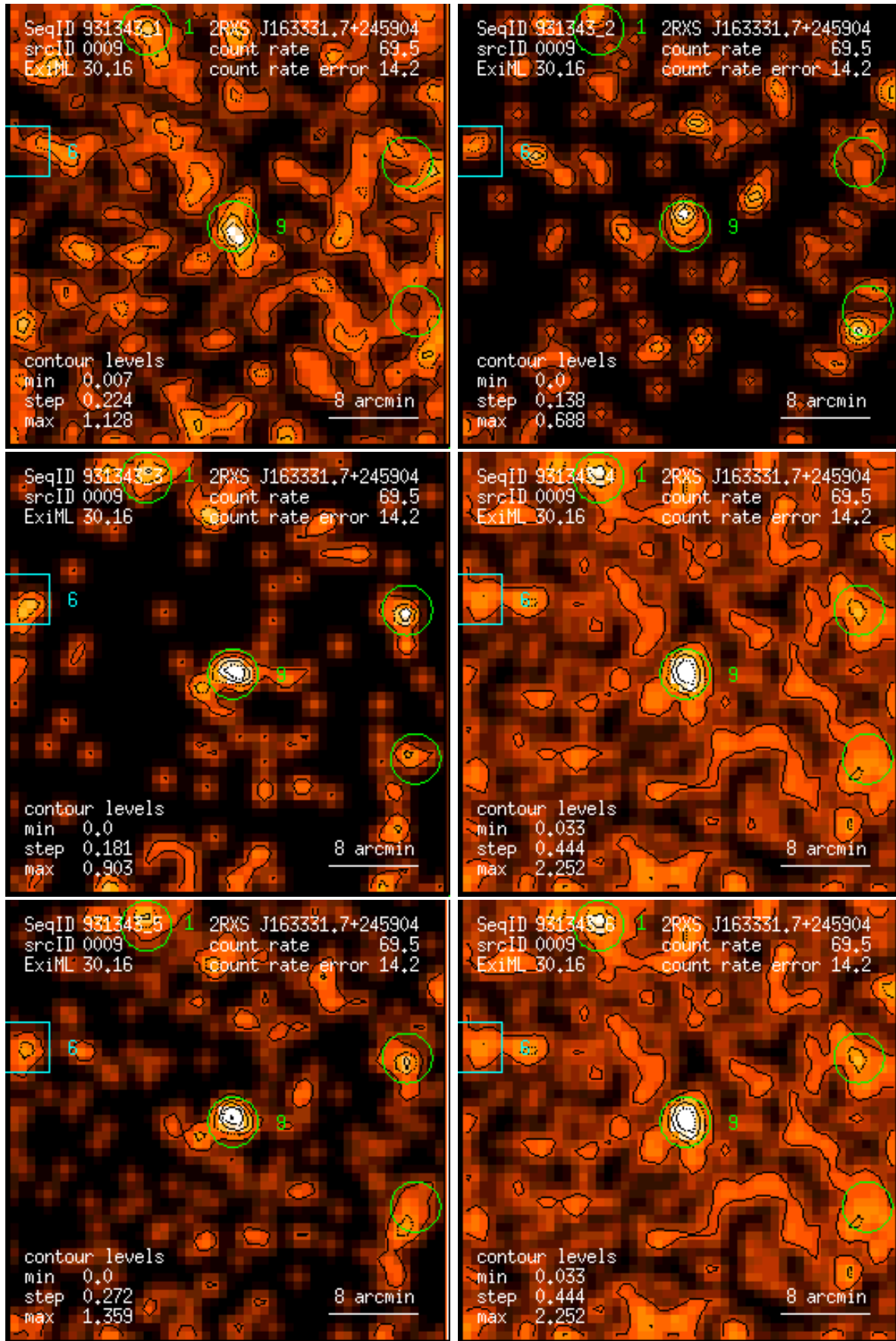
Figure 9: RASS 931343: detection 0009: band rate images, Gaussian filter: (1) PSPC channels 11 – 41, (2) 52 – 90, (3) 91 – 201, (4) 11 – 235, (5) 52 – 201, (6) 11 – 201. Broad band rates in counts/ks. Band rate contour levels in counts/ks/arcmin 2 .
