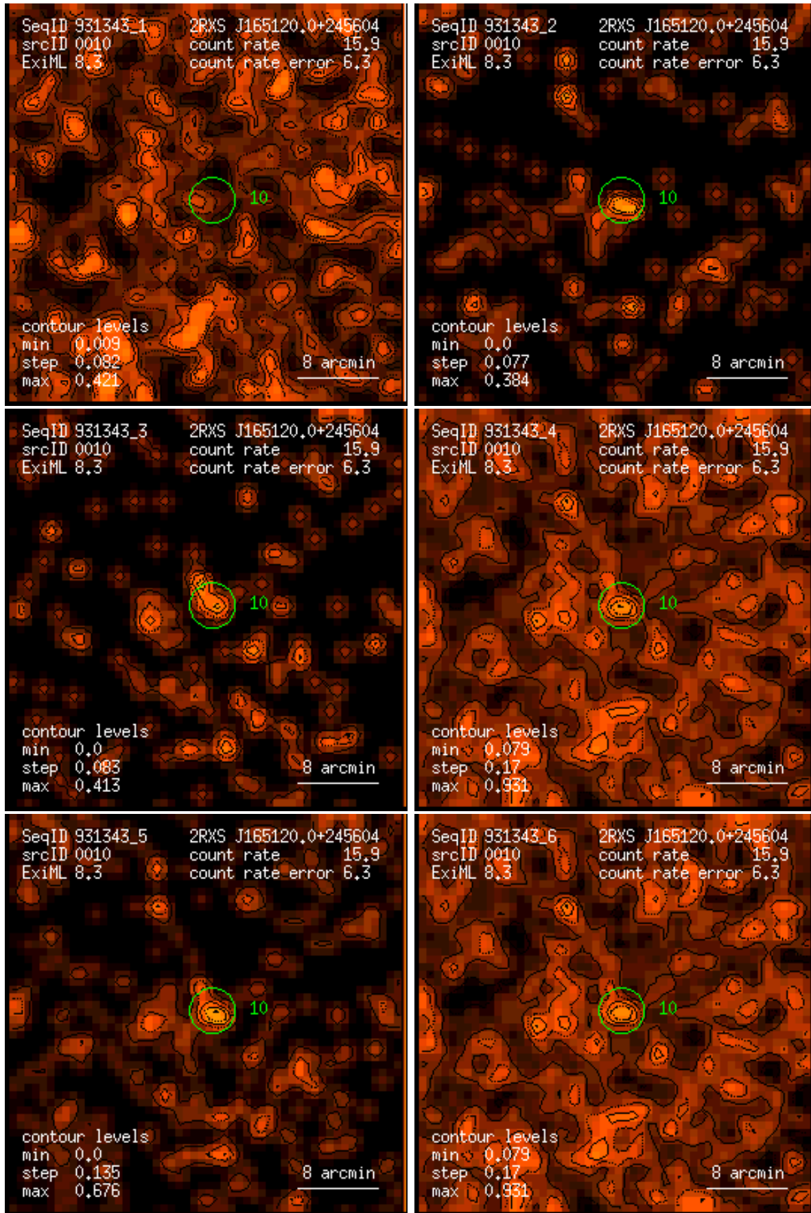
Figure 10: RASS 931343: detection 0010: band rate images, Gaussian filter: (1) PSPC channels 11 – 41, (2) 52 – 90, (3) 91 – 201, (4) 11 – 235, (5) 52 – 201, (6) 11 – 201. Broad band rates in counts/ks. Band rate contour levels in counts/ks/arcmin 2 .
