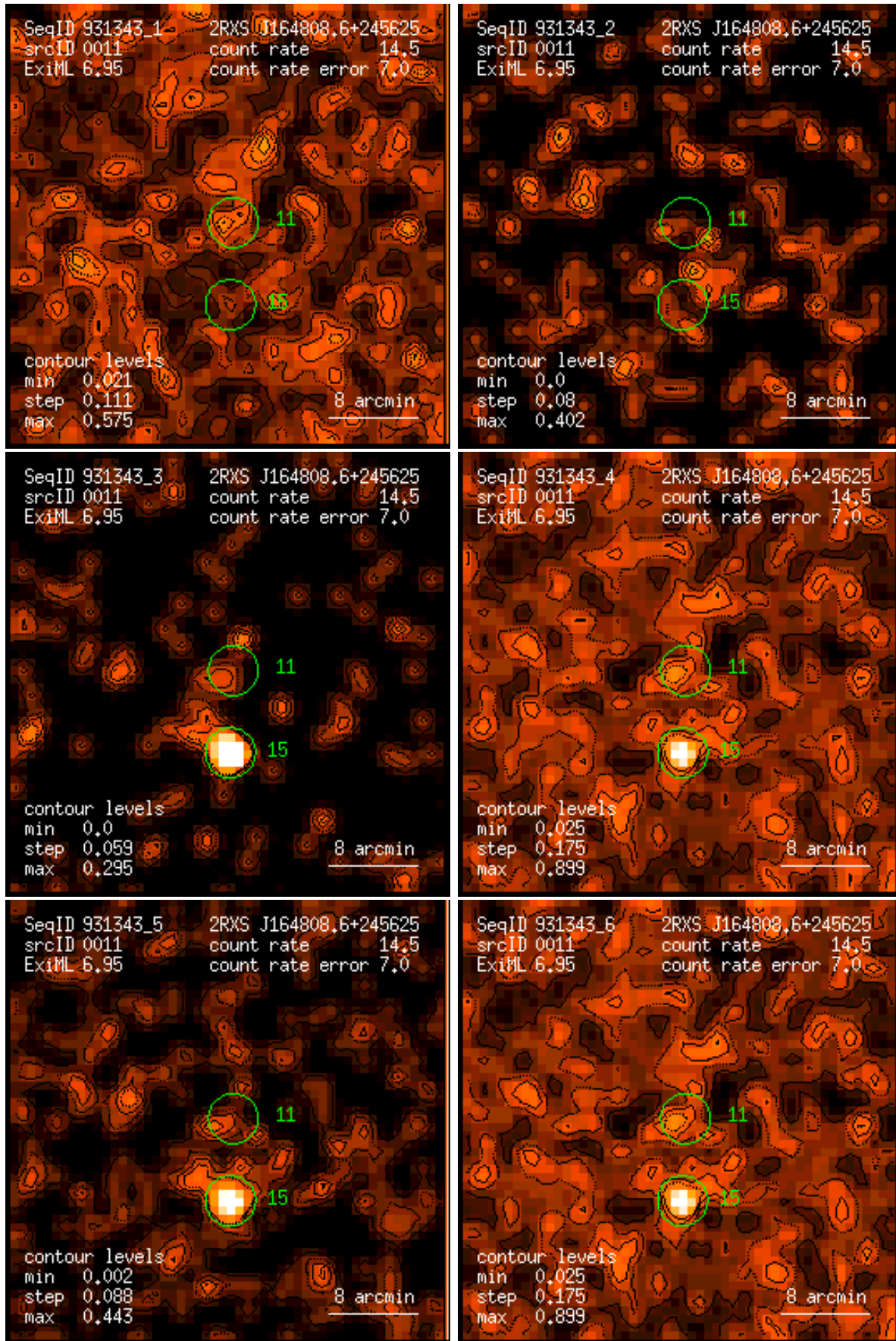
Figure 11: RASS 931343: detection 0011: band rate images, Gaussian filter: (1) PSPC channels 11 – 41, (2) 52 – 90, (3) 91 – 201, (4) 11 – 235, (5) 52 – 201, (6) 11 – 201. Broad band rates in counts/ks. Band rate contour levels in counts/ks/arcmin 2 .
