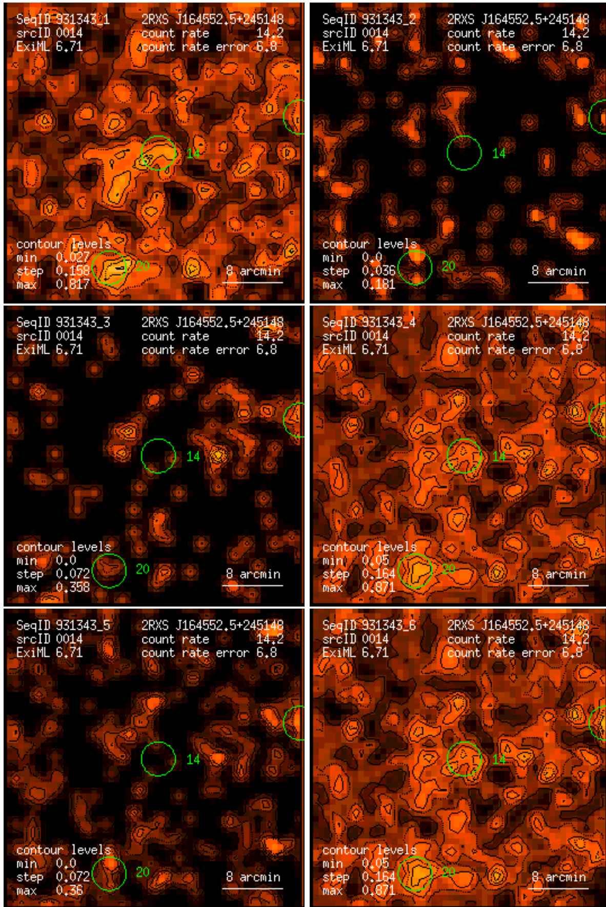
Figure 14: RASS 931343: detection 0014: band rate images, Gaussian filter: (1) PSPC channels 11 – 41, (2) 52 – 90, (3) 91 – 201, (4) 11 – 235, (5) 52 – 201, (6) 11 – 201. Broad band rates in counts/ks. Band rate contour levels in counts/ks/arcmin 2 .
