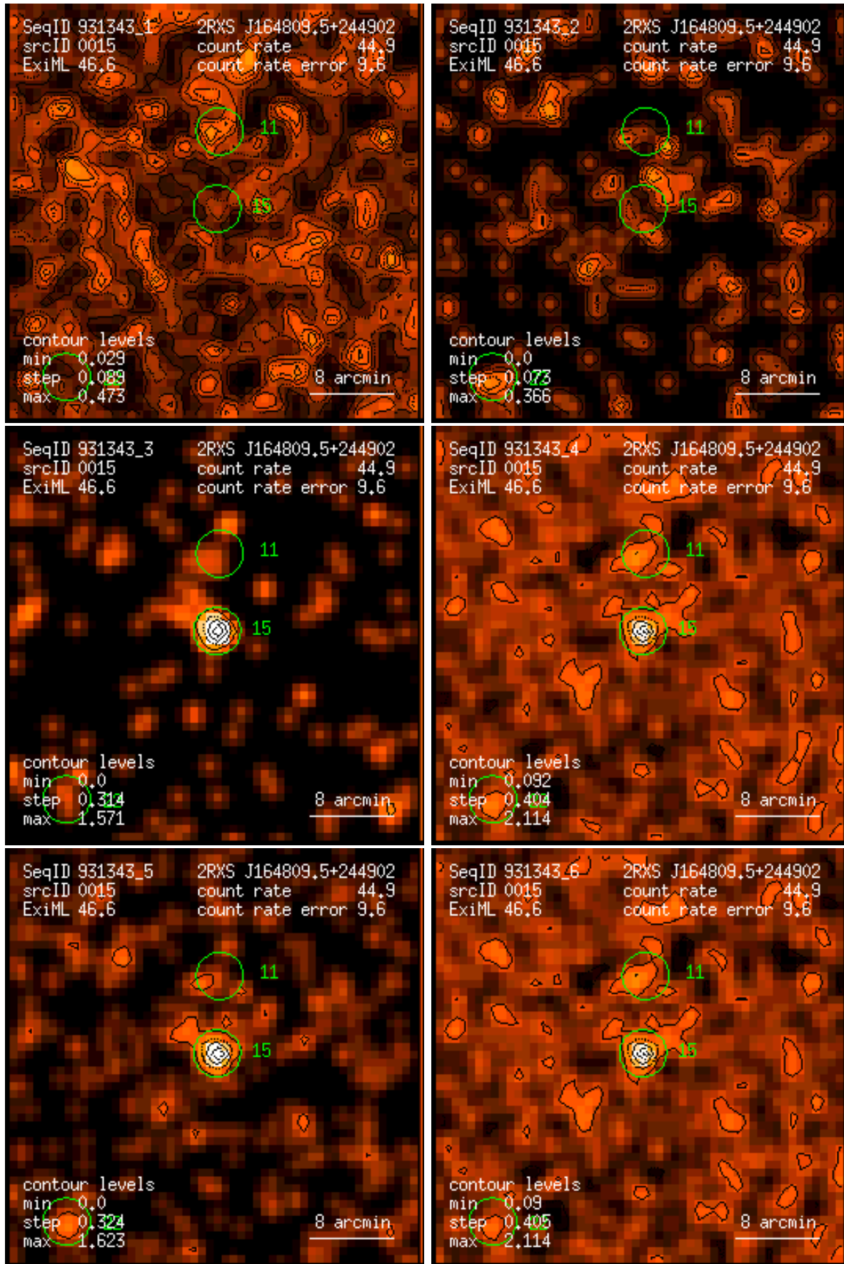
Figure 15: RASS 931343: detection 0015: band rate images, Gaussian filter: (1) PSPC channels 11 – 41, (2) 52 – 90, (3) 91 – 201, (4) 11 – 235, (5) 52 – 201, (6) 11 – 201. Broad band rates in counts/ks. Band rate contour levels in counts/ks/arcmin 2 .
