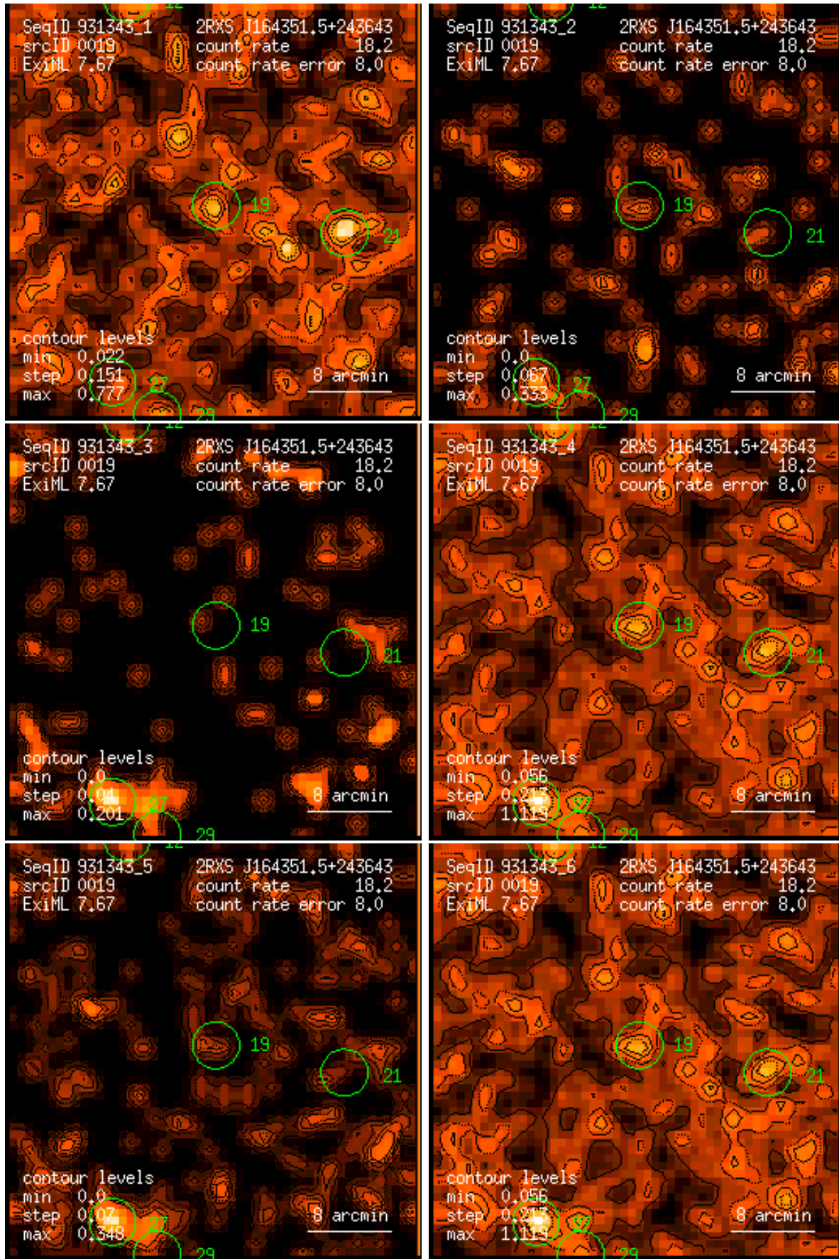
Figure 19: RASS 931343: detection 0019: band rate images, Gaussian filter: (1) PSPC channels 11 – 41, (2) 52 – 90, (3) 91 – 201, (4) 11 – 235, (5) 52 – 201, (6) 11 – 201. Broad band rates in counts/ks. Band rate contour levels in counts/ks/arcmin 2 .
