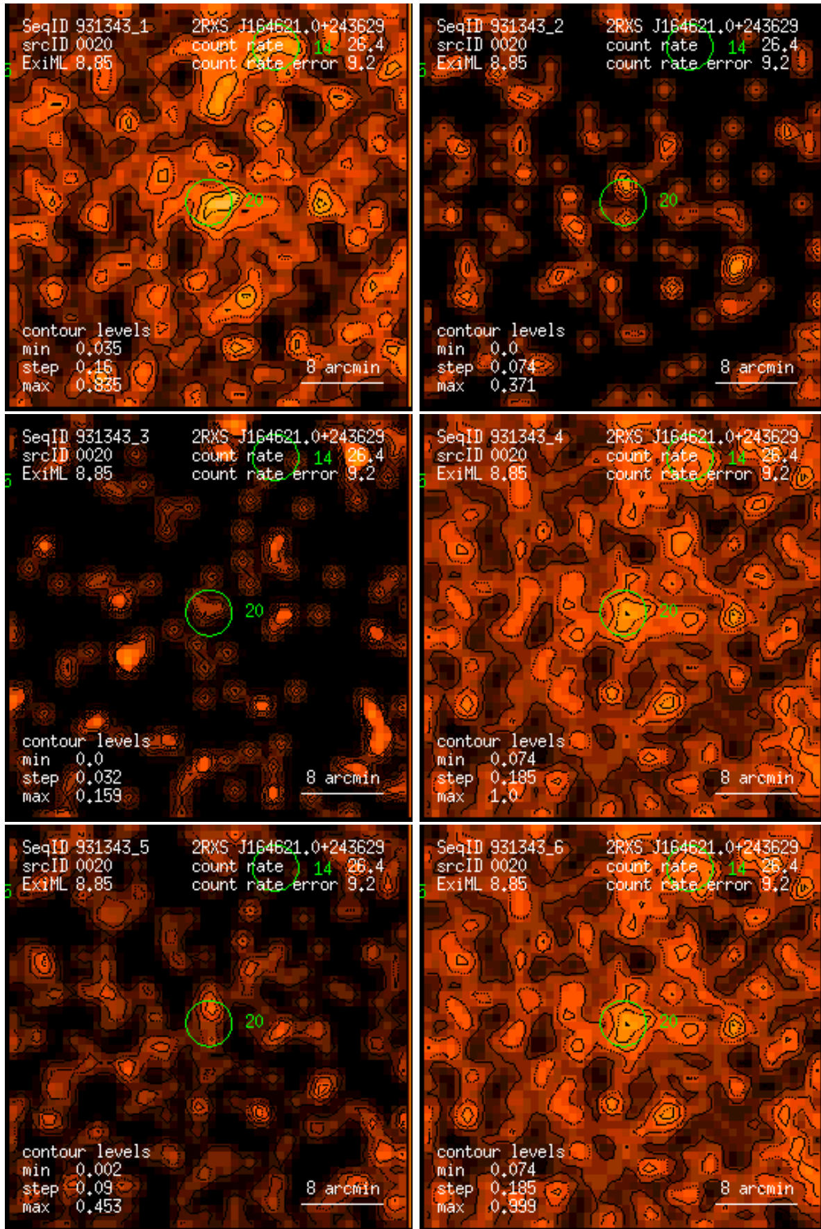
Figure 20: RASS 931343: detection 0020: band rate images, Gaussian filter: (1) PSPC channels 11 – 41, (2) 52 – 90, (3) 91 – 201, (4) 11 – 235, (5) 52 – 201, (6) 11 – 201. Broad band rates in counts/ks. Band rate contour levels in counts/ks/arcmin 2 .
