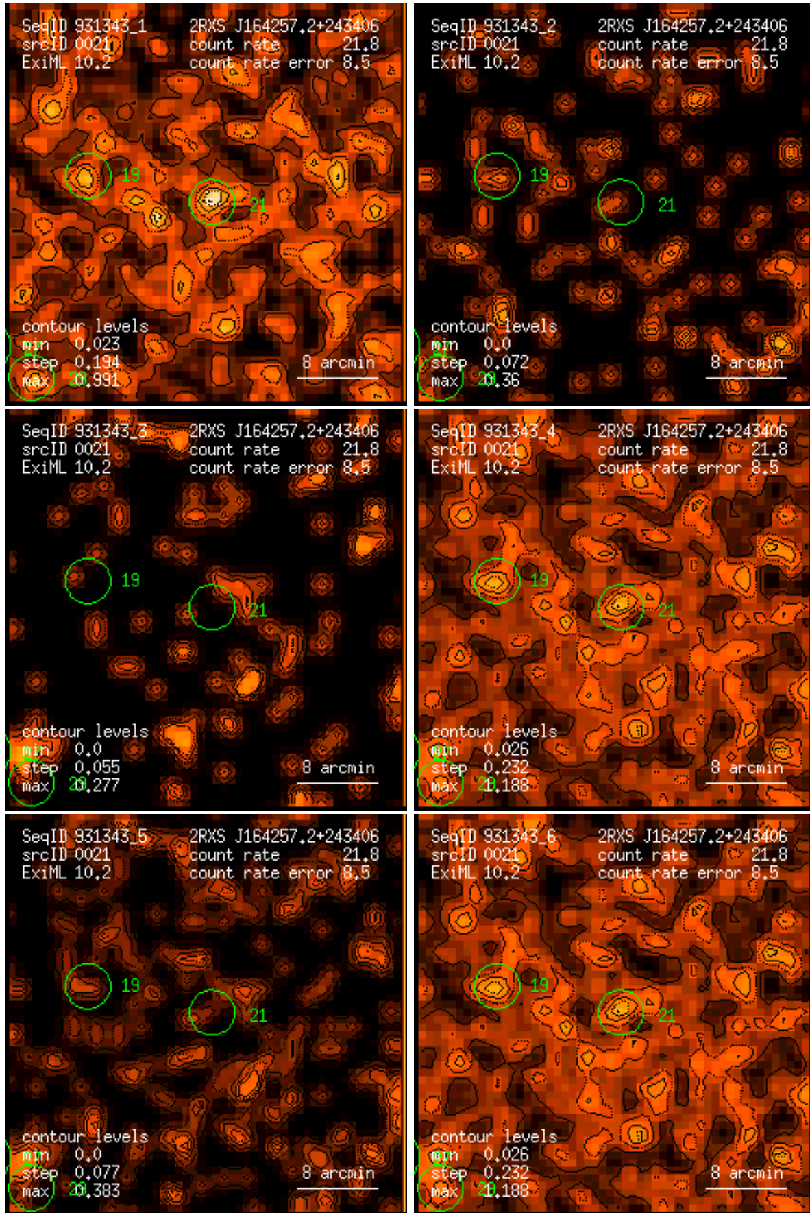
Figure 21: RASS 931343: detection 0021: band rate images, Gaussian filter: (1) PSPC channels 11 – 41, (2) 52 – 90, (3) 91 – 201, (4) 11 – 235, (5) 52 – 201, (6) 11 – 201. Broad band rates in counts/ks. Band rate contour levels in counts/ks/arcmin 2 .
