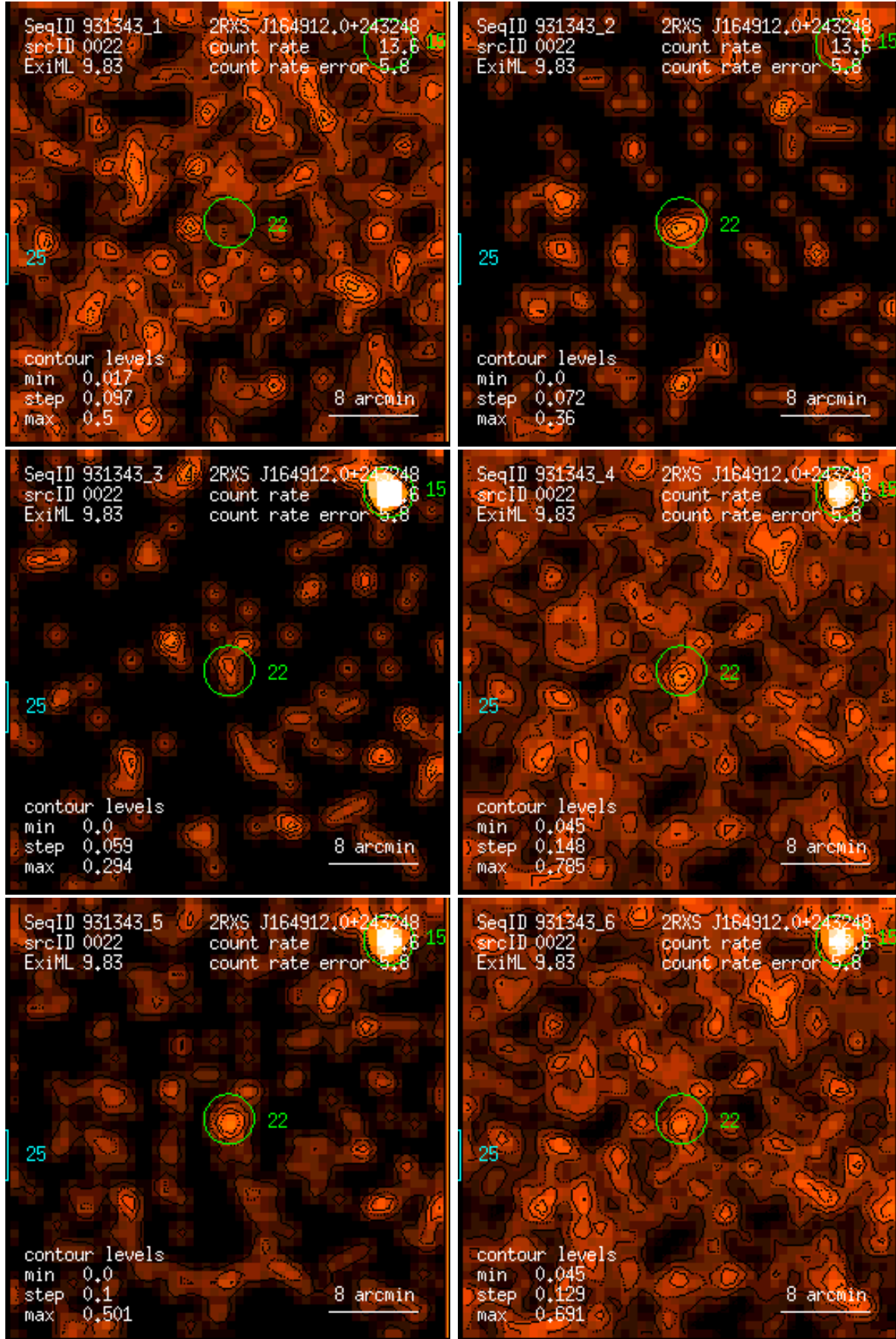
Figure 22: RASS 931343: detection 0022: band rate images, Gaussian filter: (1) PSPC channels 11 – 41, (2) 52 – 90, (3) 91 – 201, (4) 11 – 235, (5) 52 – 201, (6) 11 – 201. Broad band rates in counts/ks. Band rate contour levels in counts/ks/arcmin 2 .
