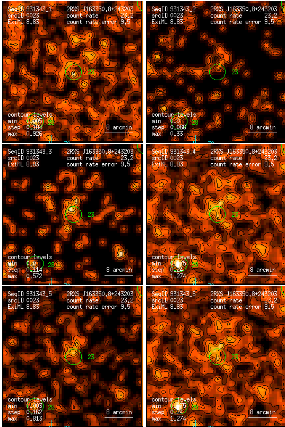
Figure 23: RASS 931343: detection 0023: band rate images, Gaussian filter: (1) PSPC channels 11 – 41, (2) 52 – 90, (3) 91 – 201, (4) 11 – 235, (5) 52 – 201, (6) 11 – 201. Broad band rates in counts/ks. Band rate contour levels in counts/ks/arcmin 2 .
