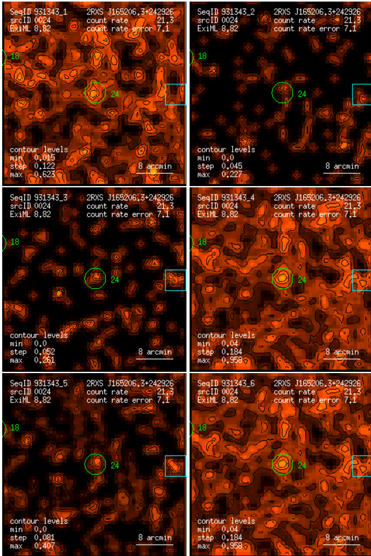
Figure 24: RASS 931343: detection 0024: band rate images, Gaussian filter: (1) PSPC channels 11 – 41, (2) 52 – 90, (3) 91 – 201, (4) 11 – 235, (5) 52 – 201, (6) 11 – 201. Broad band rates in counts/ks. Band rate contour levels in counts/ks/arcmin 2 .
