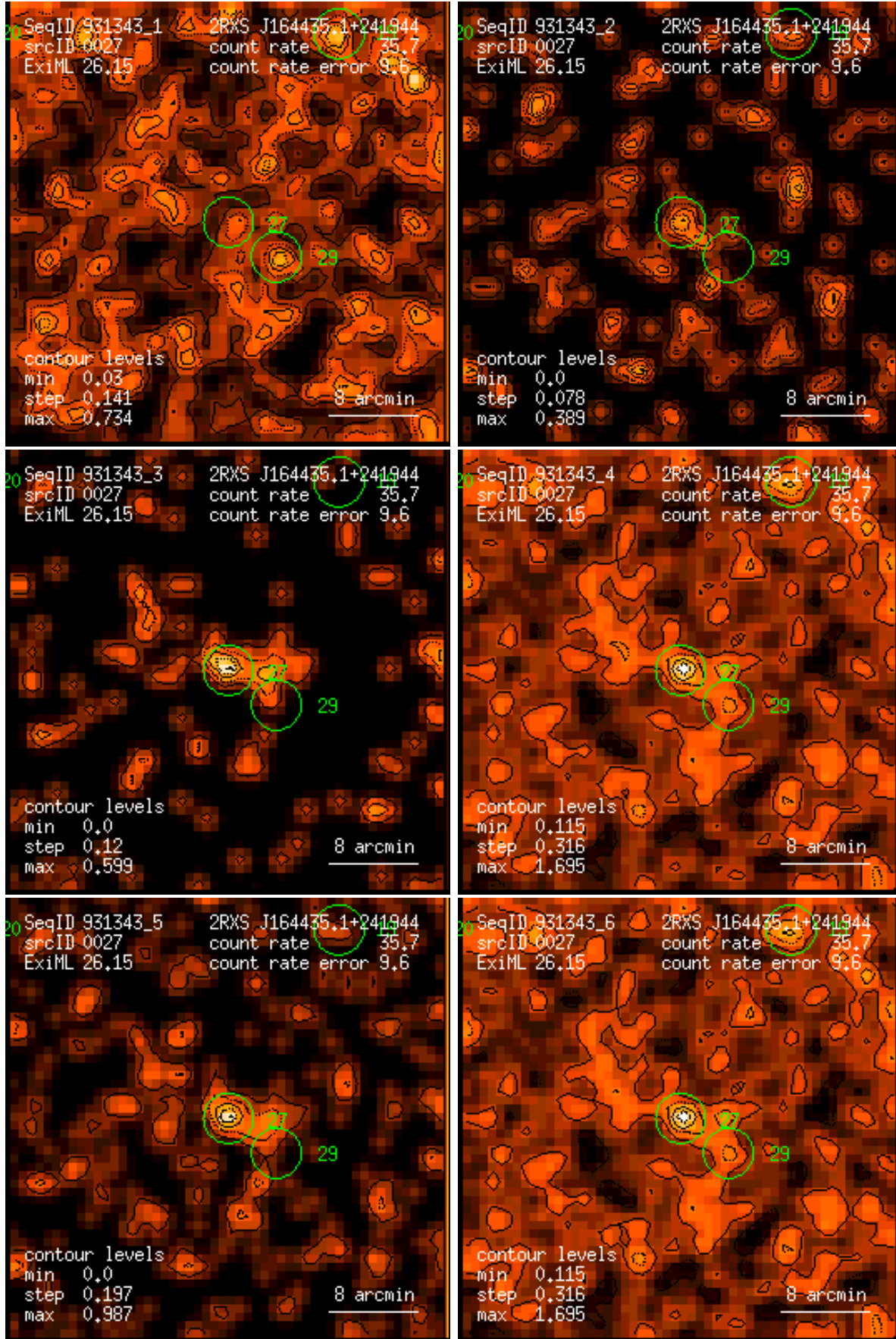
Figure 27: RASS 931343: detection 0027: band rate images, Gaussian filter: (1) PSPC channels 11 – 41, (2) 52 – 90, (3) 91 – 201, (4) 11 – 235, (5) 52 – 201, (6) 11 – 201. Broad band rates in counts/ks. Band rate contour levels in counts/ks/arcmin 2 .
