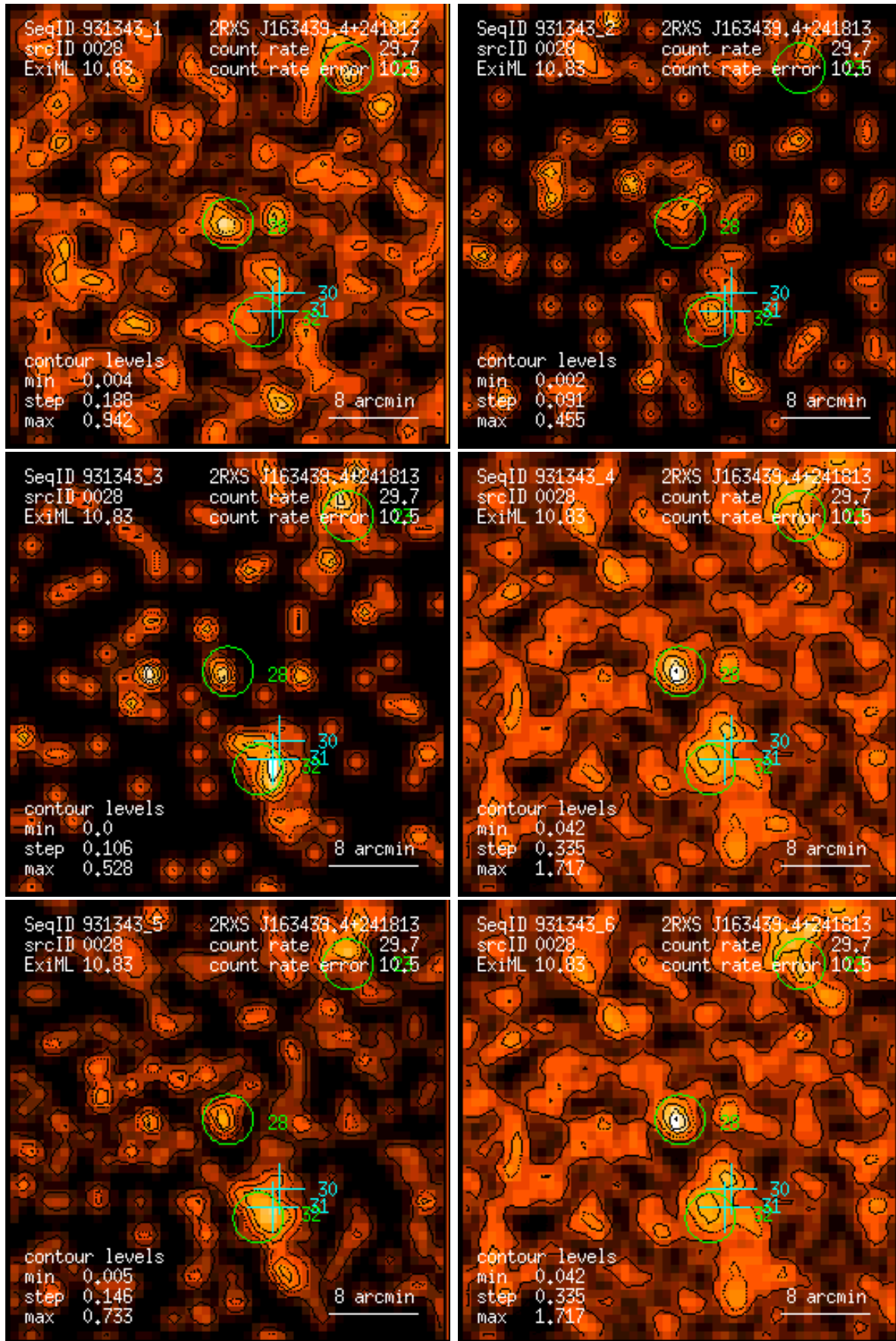
Figure 28: RASS 931343: detection 0028: band rate images, Gaussian filter: (1) PSPC channels 11 – 41, (2) 52 – 90, (3) 91 – 201, (4) 11 – 235, (5) 52 – 201, (6) 11 – 201. Broad band rates in counts/ks. Band rate contour levels in counts/ks/arcmin 2 .
