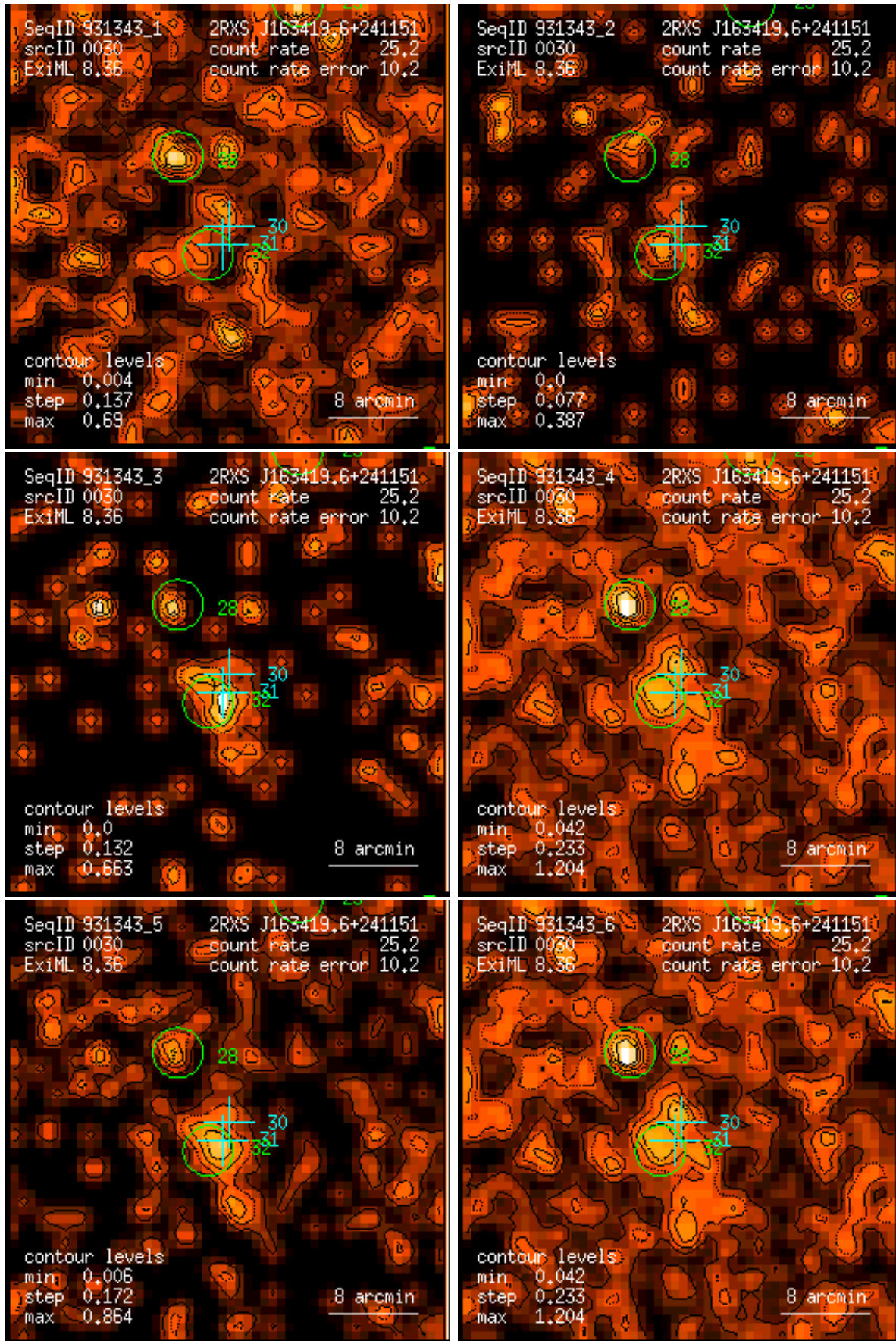
Figure 30: RASS 931343: detection 0030: band rate images, Gaussian filter: (1) PSPC channels 11 – 41, (2) 52 – 90, (3) 91 – 201, (4) 11 – 235, (5) 52 – 201, (6) 11 – 201. Broad band rates in counts/ks. Band rate contour levels in counts/ks/arcmin 2 .
