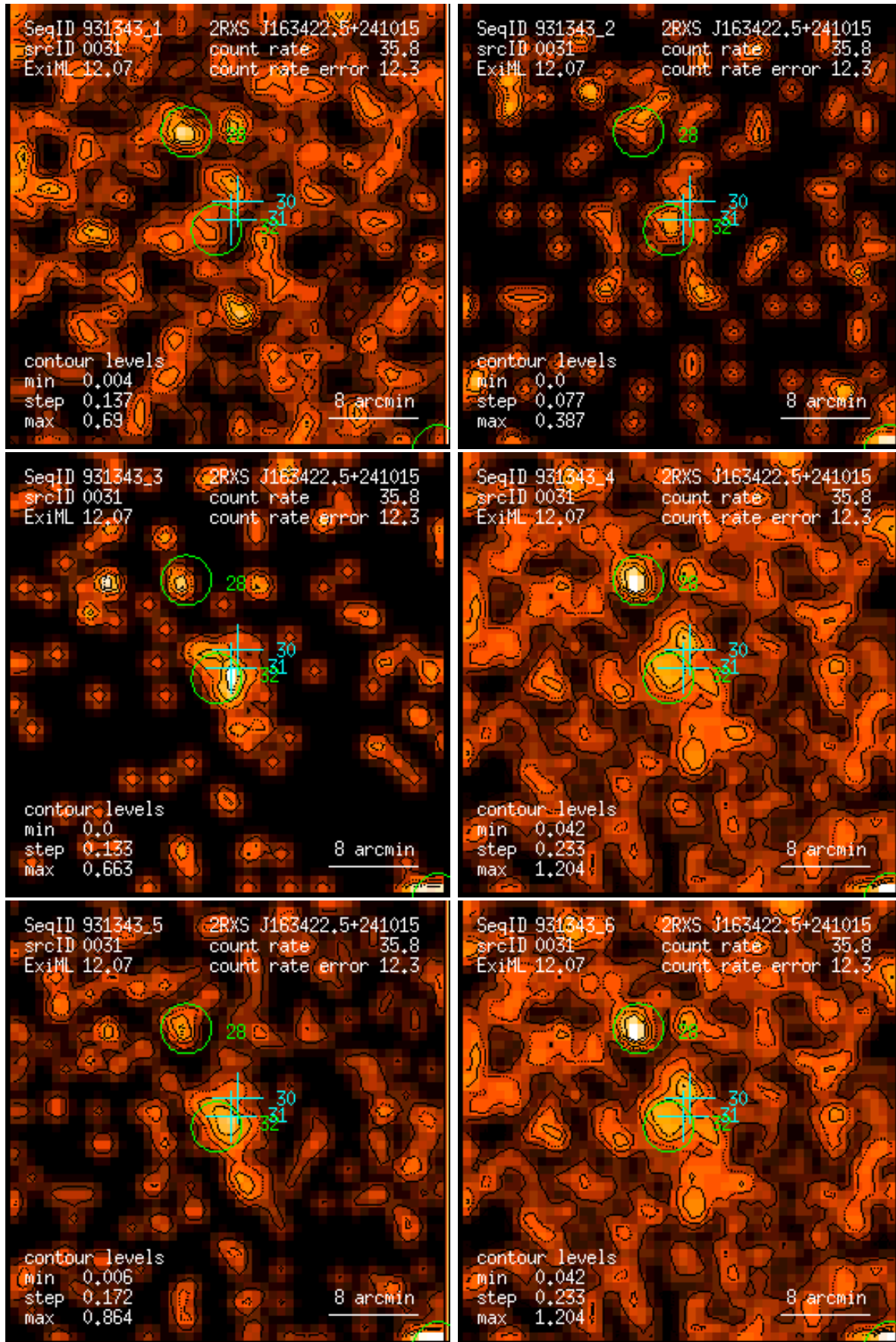
Figure 31: RASS 931343: detection 0031: band rate images, Gaussian filter: (1) PSPC channels 11 – 41, (2) 52 – 90, (3) 91 – 201, (4) 11 – 235, (5) 52 – 201, (6) 11 – 201. Broad band rates in counts/ks. Band rate contour levels in counts/ks/arcmin 2 .
