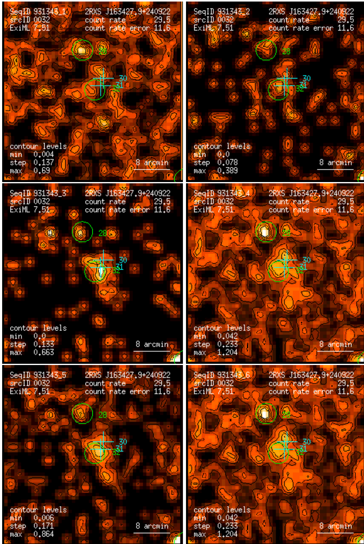
Figure 32: RASS 931343: detection 0032: band rate images, Gaussian filter: (1) PSPC channels 11 – 41, (2) 52 – 90, (3) 91 – 201, (4) 11 – 235, (5) 52 – 201, (6) 11 – 201. Broad band rates in counts/ks. Band rate contour levels in counts/ks/arcmin 2 .
